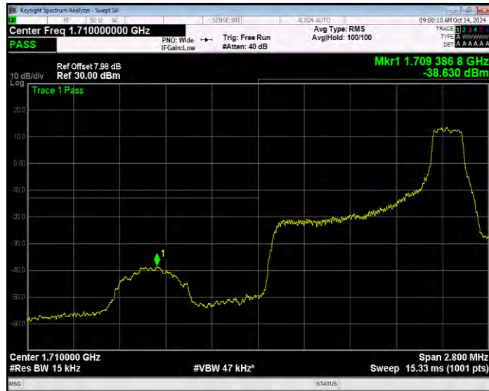
Band4 QPSK BW=1.4MHz Channel=19957 RB Size=6 Position=#0 Extended
