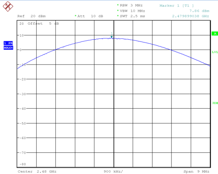
Fig.9 Peak Conducted Output Power CH78, 3DH1
