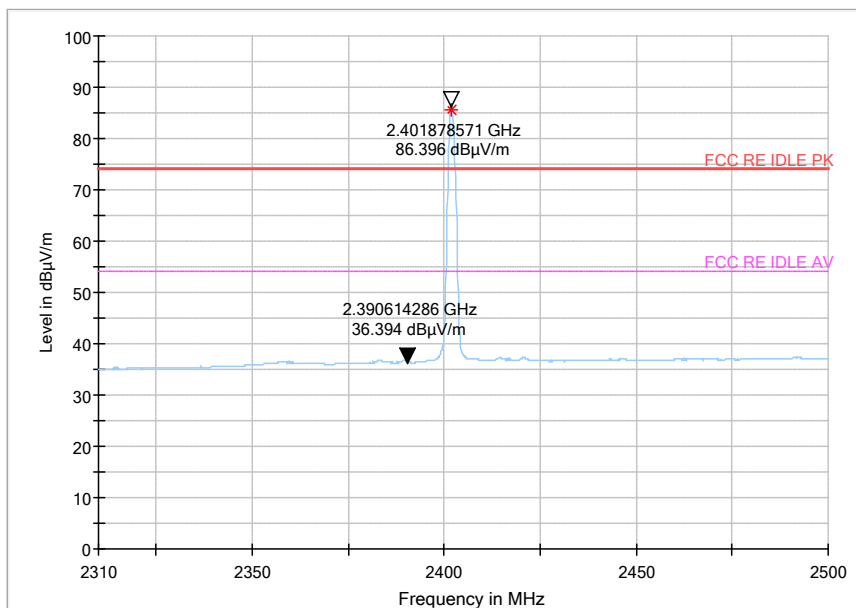
Fig.53 Radiated emission (Power): \pi/4 DQPSK, low channel
