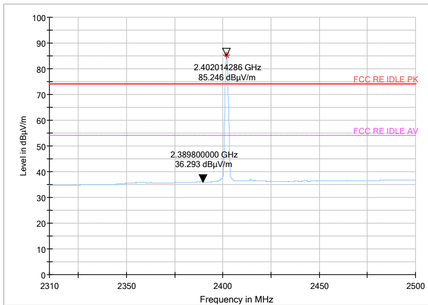
Fig.48 Radiated emission (Power): GFSK, low channel
