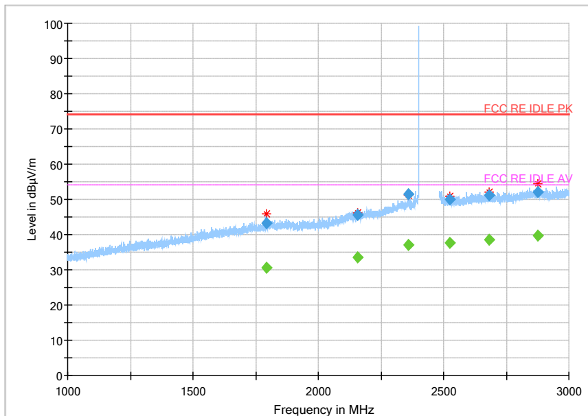
Fig.51 Radiated emission: \pi/4 DQPSK, Ch0, 1GHz~3GHz
