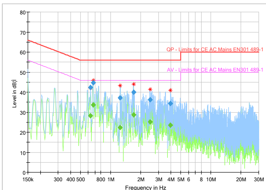
Fig.96 AC Powerline Conducted Emission
