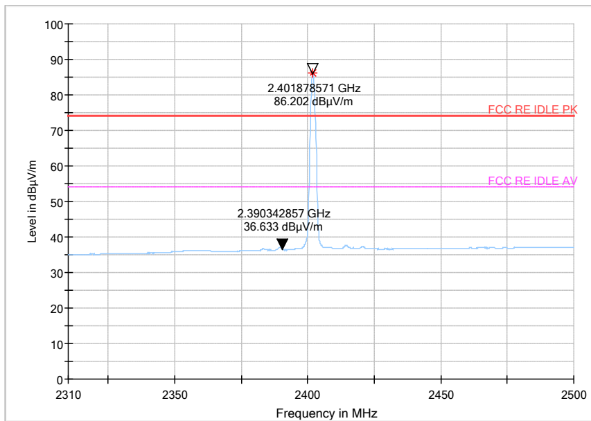
Fig.58 Radiated emission (Power): 8DPSK, low channel
