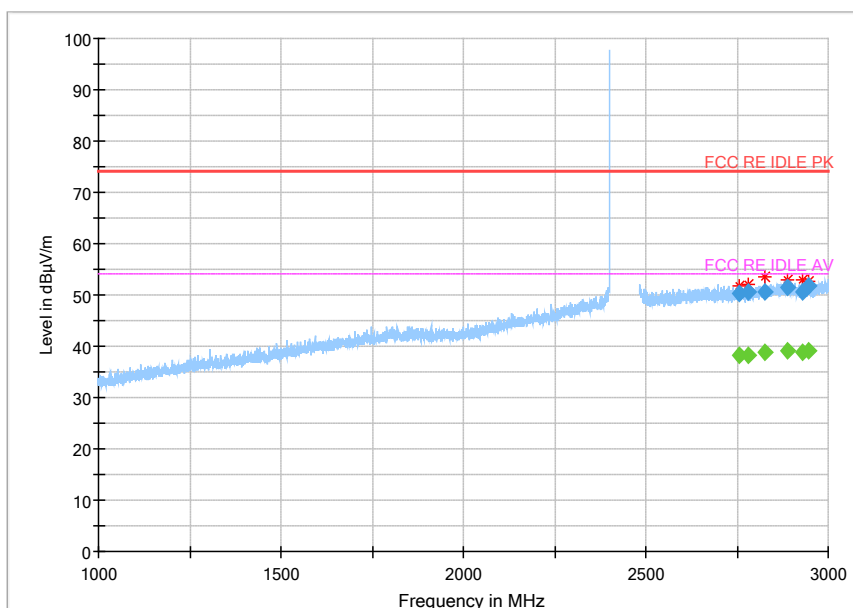
Fig.46 Radiated emission: GFSK, Ch0, 1GHz~3GHz
