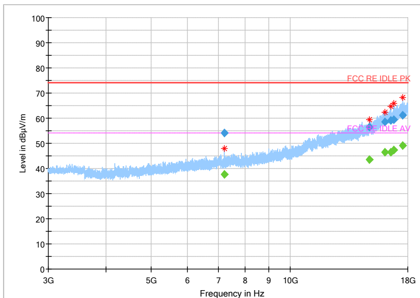
Fig.57 Radiated emission: 8DPSK, Ch0, 3GHz~18GHz
