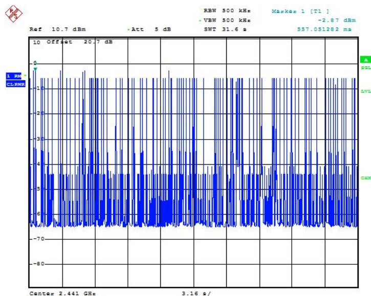
Fig.64 Time of occupancy (Dwell Time): Ch39,Packet DH5
