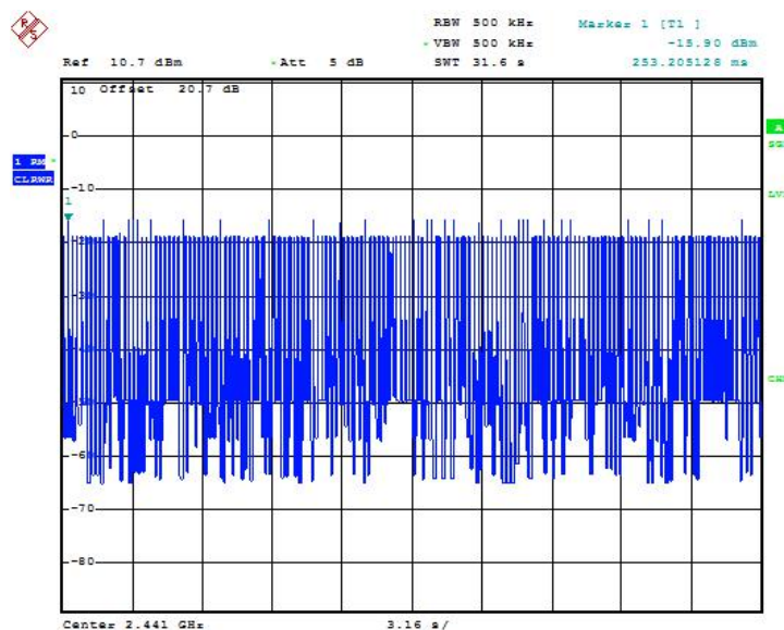
Fig.72 Time of occupancy (Dwell Time): Ch39,Packet 3-DH1
