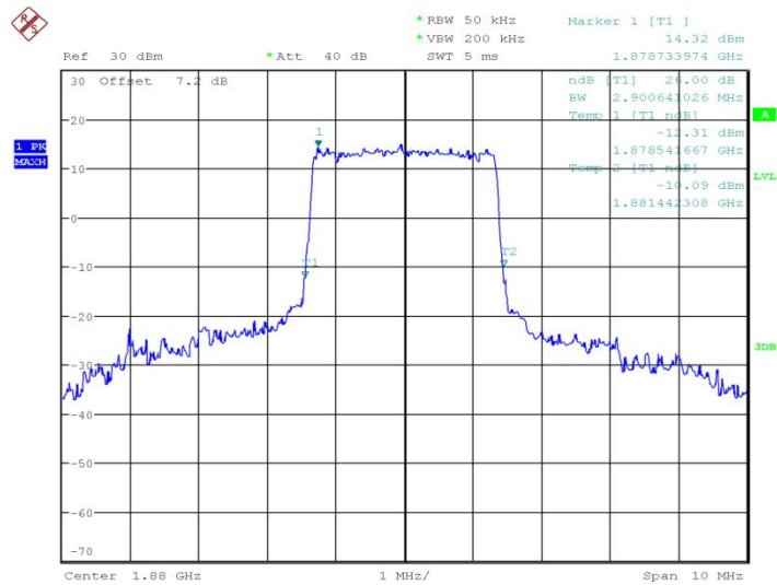
LTE band 2, 3MHz Bandwidth, QPSK (-26dBc BW)
