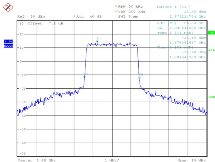
LTE band 2, 3MHz Bandwidth, 16QAM (-26dBc BW)
