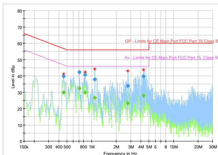
Fig.24 AC Powerline Conducted Emission
