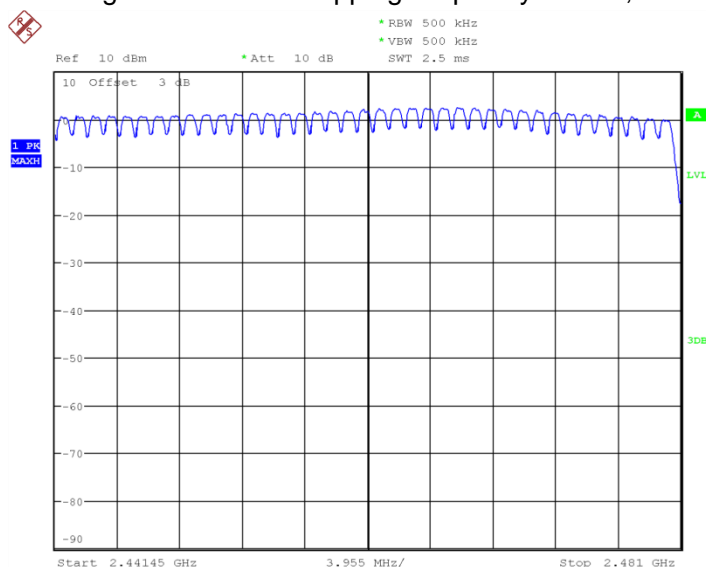
Fig.79 Number of hopping frequency: GFSK, Ch0~39
