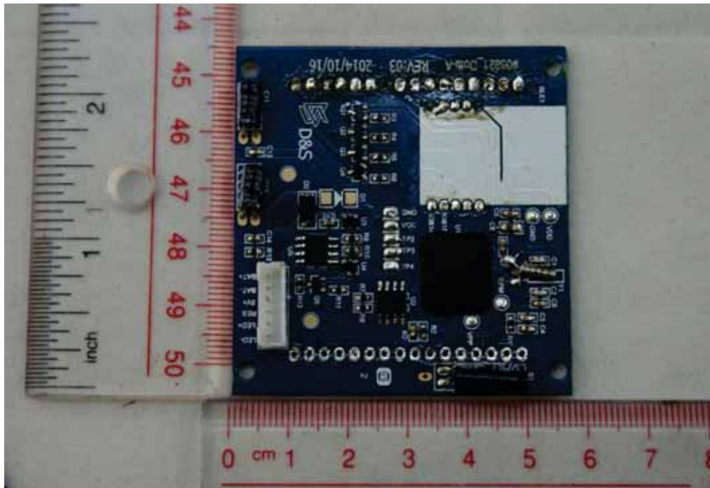
EUT MAIN BOARD TOP VIEW 4
