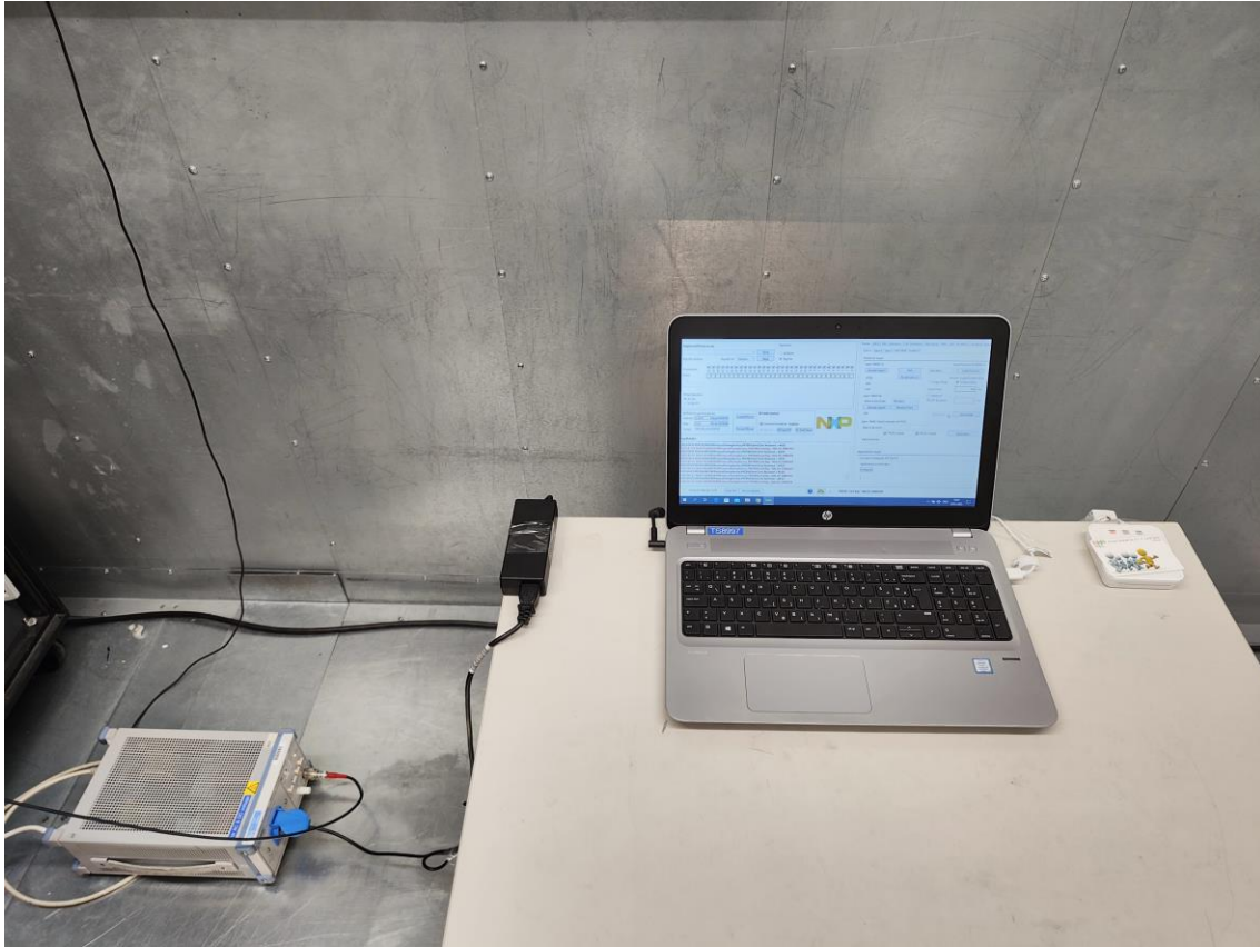
Figure 3: Conducted emission
