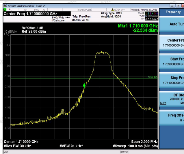
Band4-1.4MHz-QPSK-19957-1RB#5
