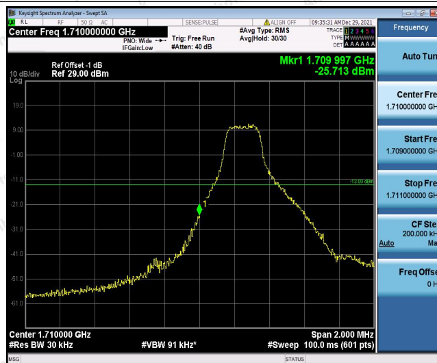
Band4-1.4MHz-16QAM-19957-1RB#5
