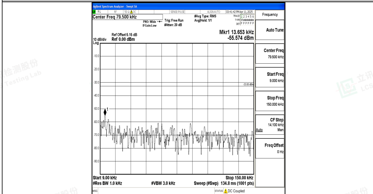
Band12_10MHz_16QAM_23130_1RB#0_0.009~0.15_0.009~0.15
