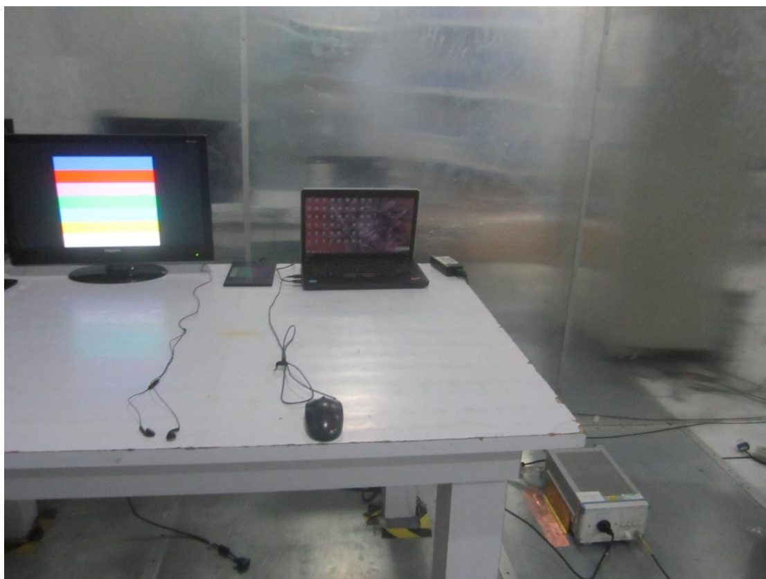
Conducted Emission Test setup photo
