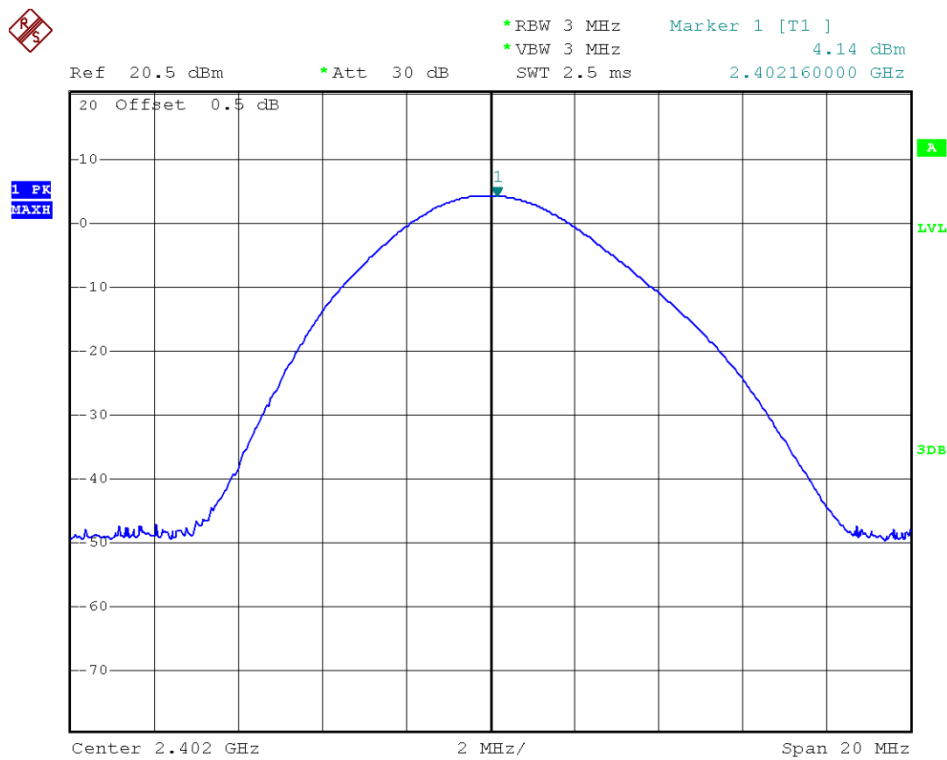
Plot C1: 8-DPSK
