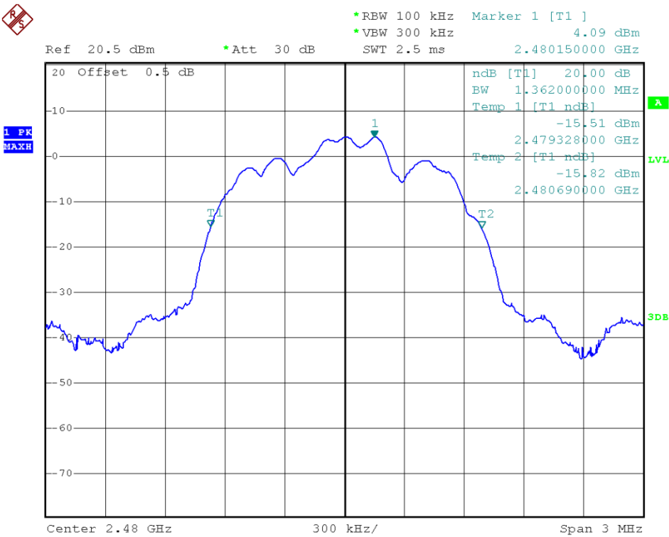
(Plot F: Channel = 2480 @ \pi/4 -DQPSK)
