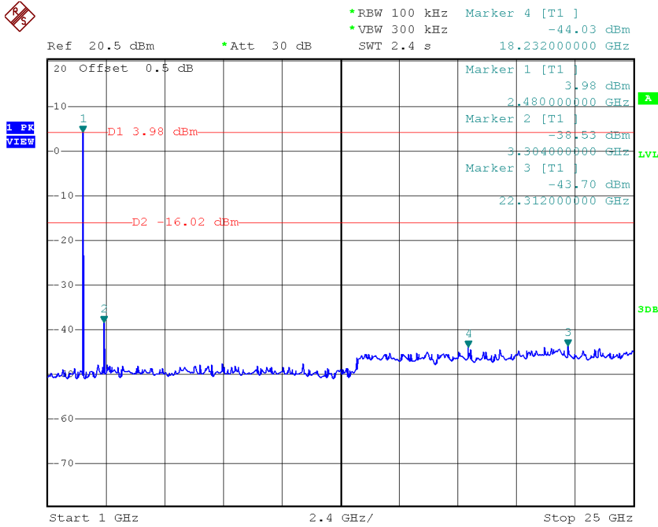
(Plot C.2: Channel = 78, 1GHz to 25GHz @ GFSK Mode)
