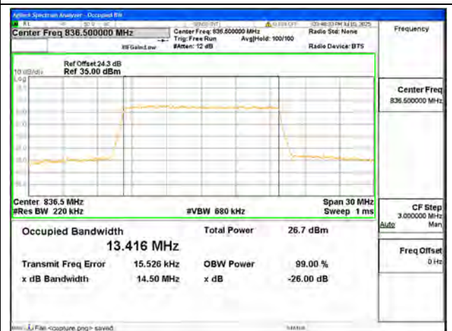
B26 / 15MHz / 64QAM/ Mid CH
