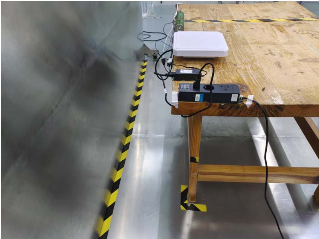
AC Line Conducted Emissions Side View M1
