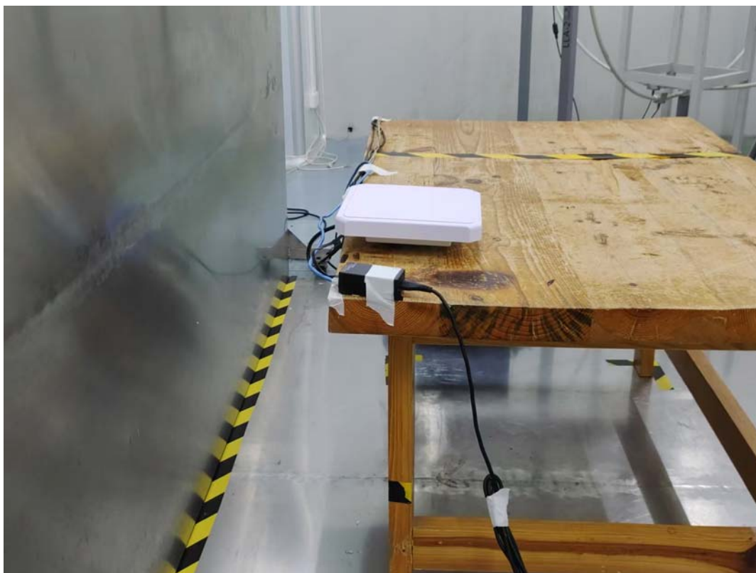
AC Line Conducted Emissions Side View M2
