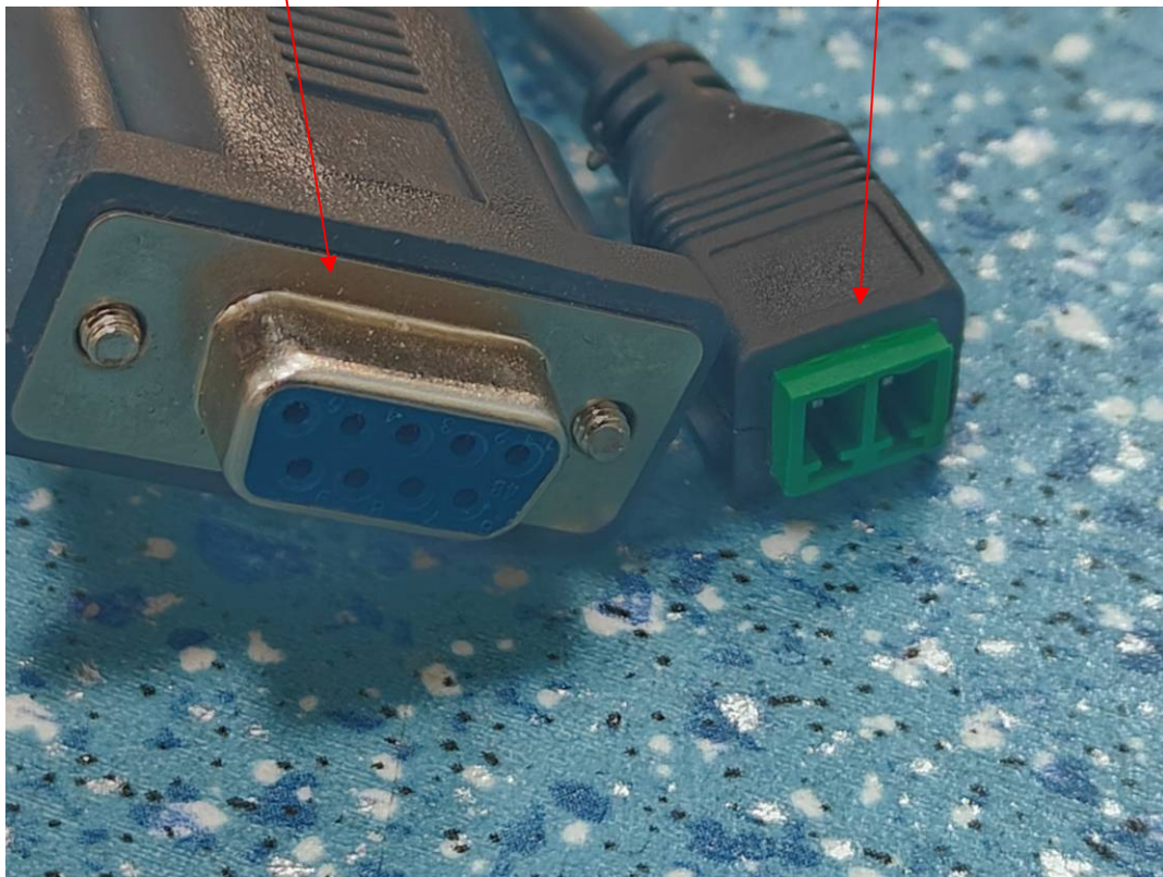
RS232 Interface
