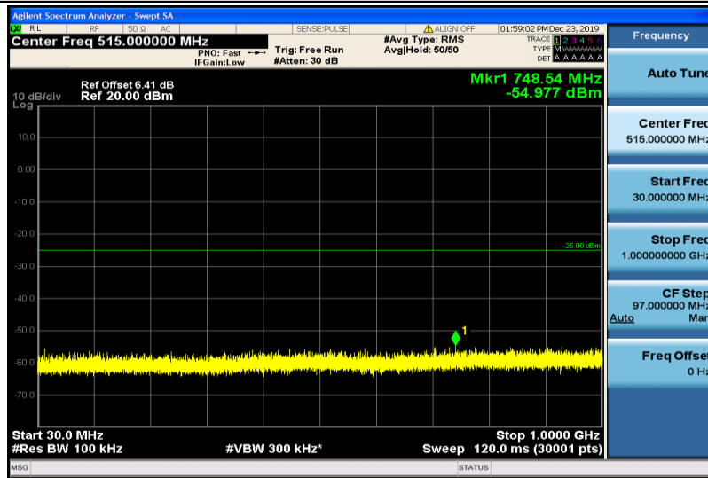
Band41-5MHz-16QAM-40740-1RB#0-30~1000MHz
