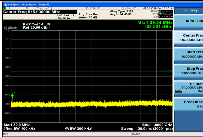
Band41-10MHz-QPSK-40740-1RB#0-30~1000MHz
