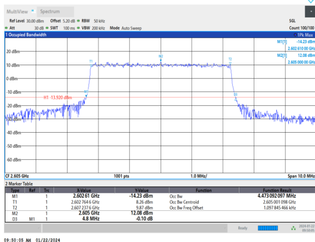
Band41-5MHz-16QAM-40740-25RB#0
