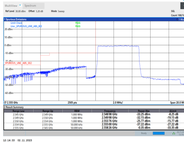
Band41-5MHz-QPSK-40265-25RB#0
