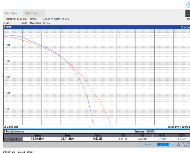
Band38-20MHz-QPSK-38000-100RB#0
