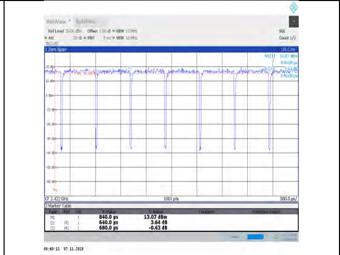
NTNV-11n40SISO-Ant2-2422
