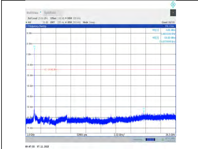
11n20SISO-Ant2-2462-1000~26500-PASS
