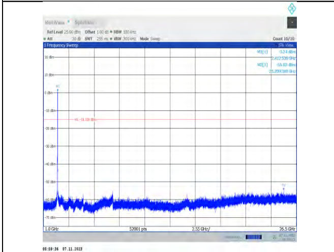
11n20SISO-Ant2-2412-1000~26500-PASS
