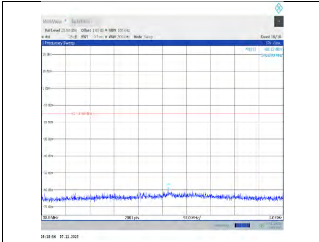
11n20SISO-Ant2-2437-30~1000-PASS
