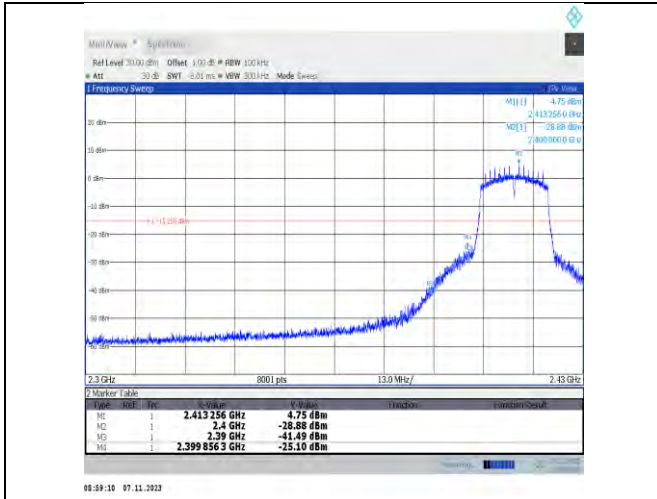
11n20SISO-Ant2-2412-PASS
