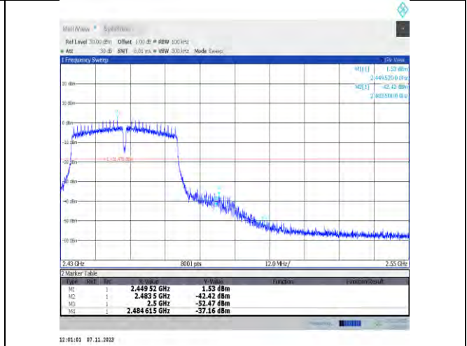
11n40SISO-Ant2-2452-PASS
