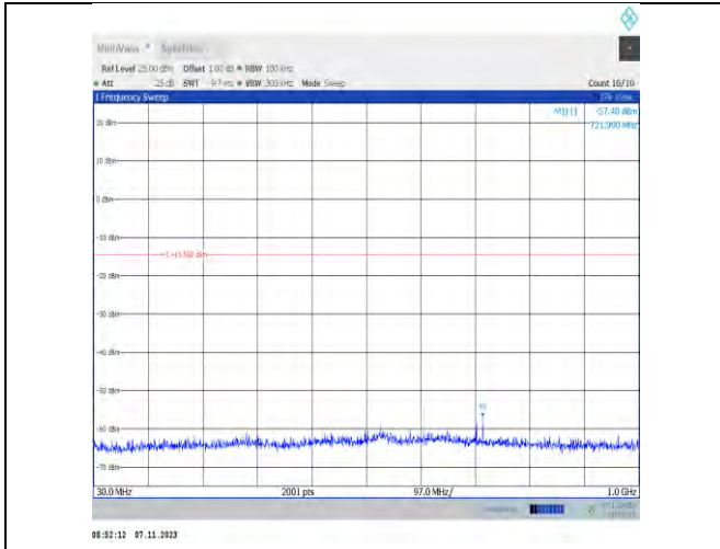
11g-Ant2-2462-30~1000-PASS
