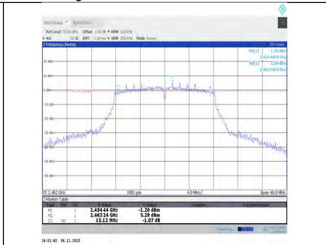
11g-Ant2-2462-PASS
