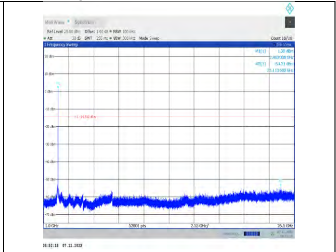
11g-Ant2-2462-1000~26500-PASS
