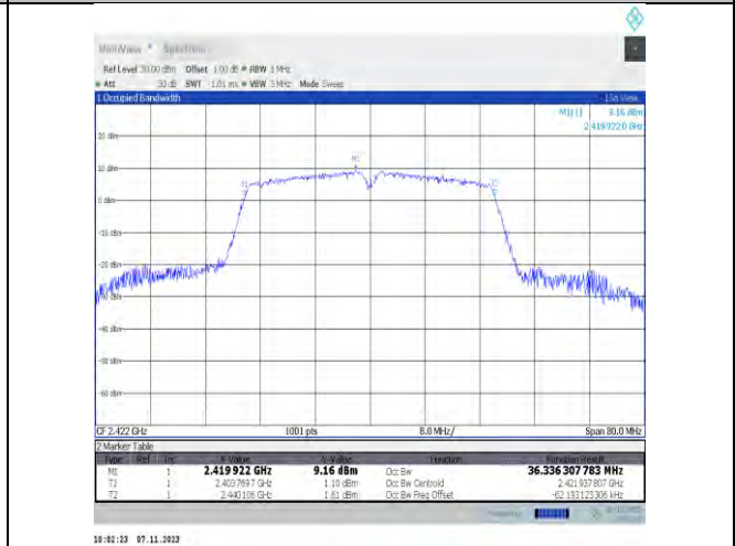
11n40SISO-Ant2-2422
