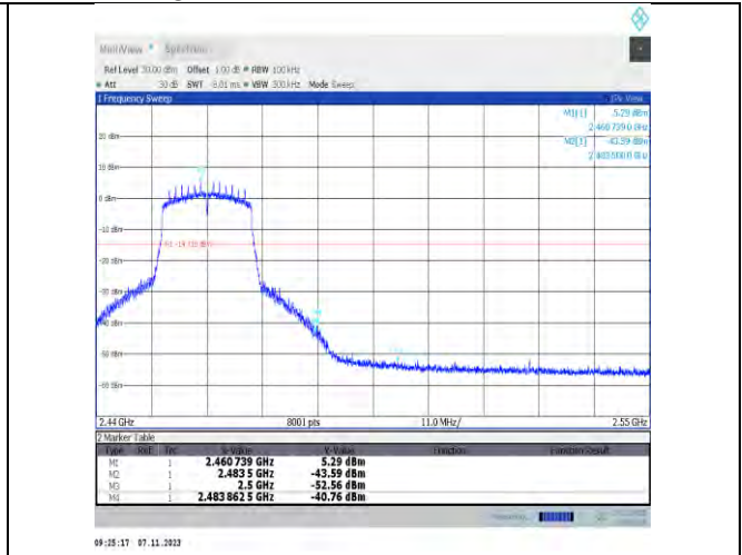
11n20SISO-Ant2-2462-PASS
