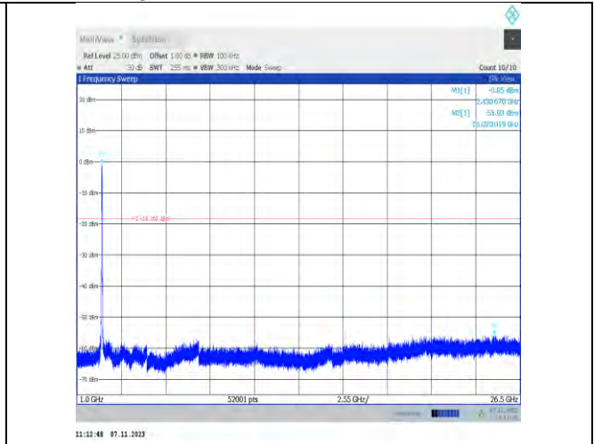
11n40SISO-Ant2-2422-1000~26500-PASS
