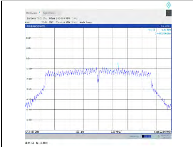
11g-Ant2-2437-PASS
