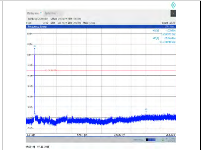
11n20SISO-Ant2-2437-1000~26500-PASS
