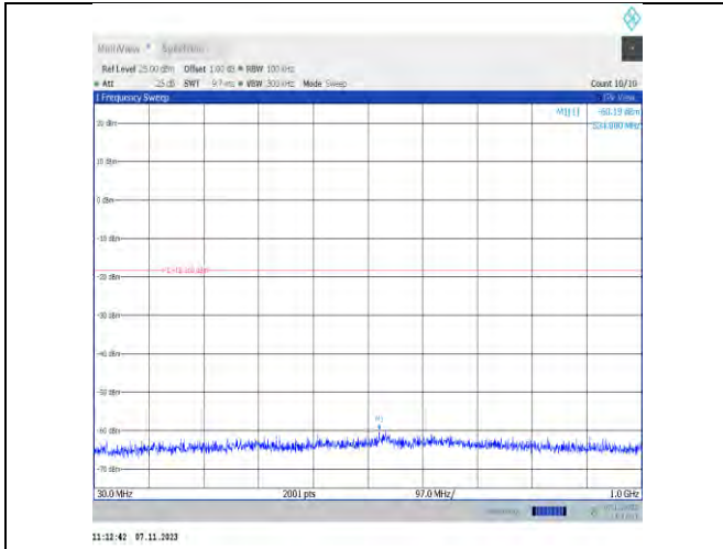
11n40SISO-Ant2-2422-30~1000-PASS
