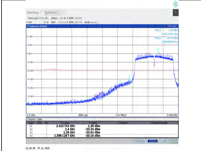
11n40SISO-Ant2-2422-PASS
