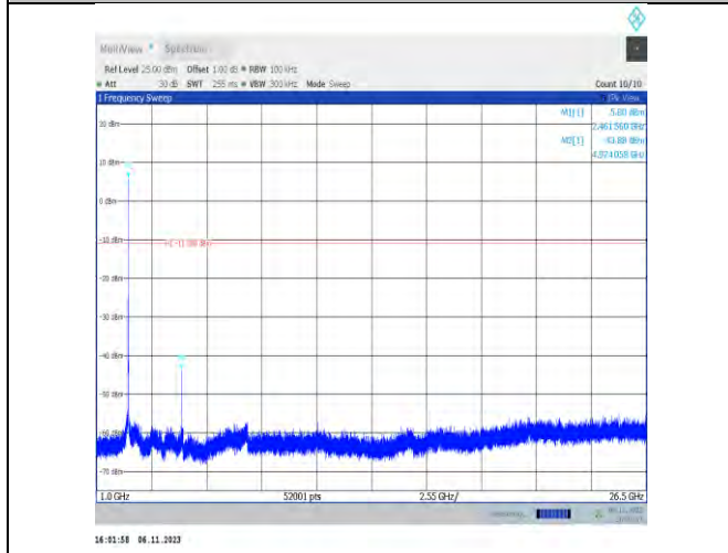
11b-Ant2-2462-1000~26500-PASS
