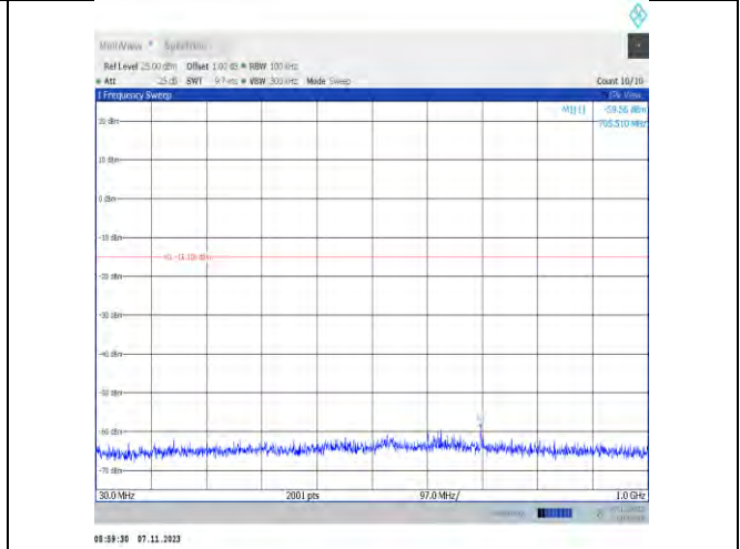
11n20SISO-Ant2-2412-30~1000-PASS
