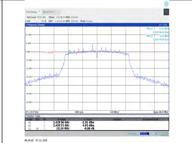
11n20SISO-Ant2-2437-PASS
