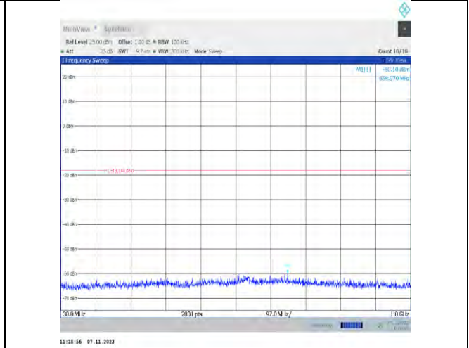
11n40SISO-Ant2-2437-30~1000-PASS
