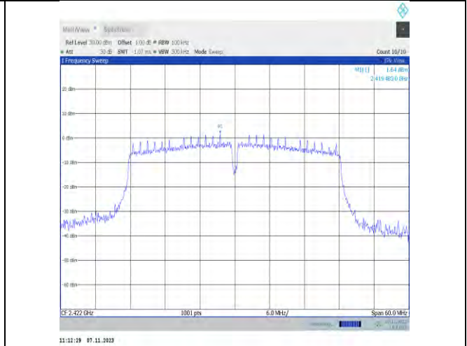
11n40SISO-Ant2-2422-0~Reference-PASS
