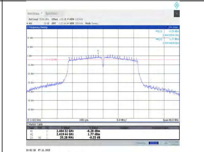
11n40SISO-Ant2-2422-PASS
