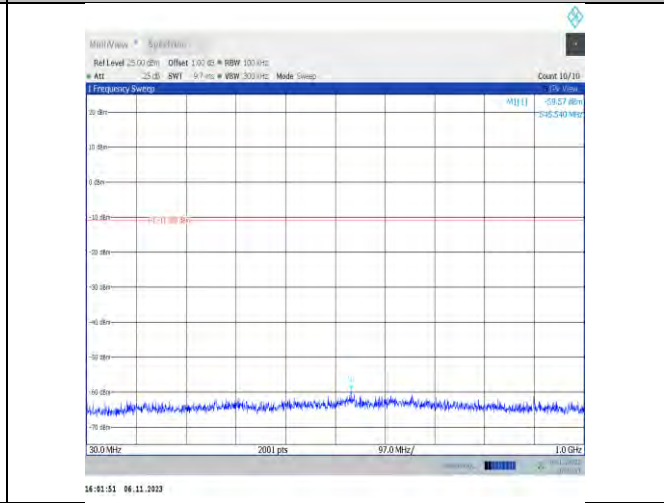
11b-Ant2-2462-30~1000-PASS
