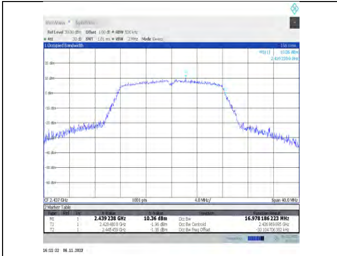
11g-Ant2-2437
