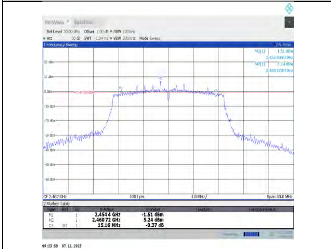
11n20SISO-Ant2-2462-PASS
