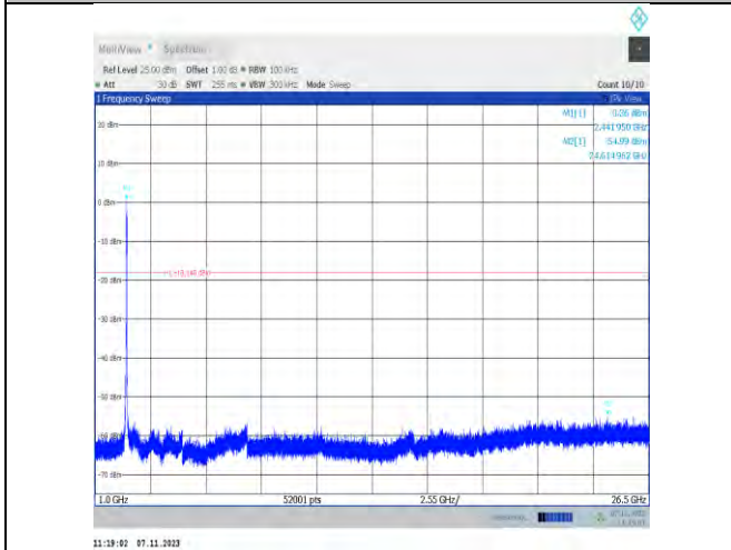
11n40SISO-Ant2-2437-1000~26500-PASS
