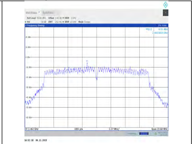
11g-Ant2-2462-PASS
