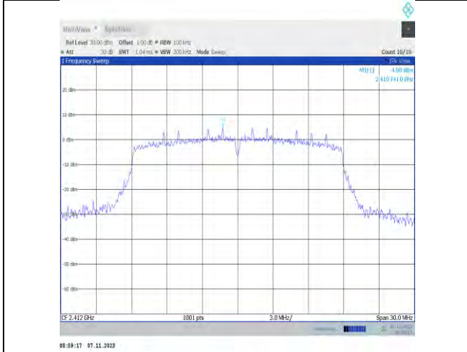
11n20SISO-Ant2-2412-0-Reference-PASS
