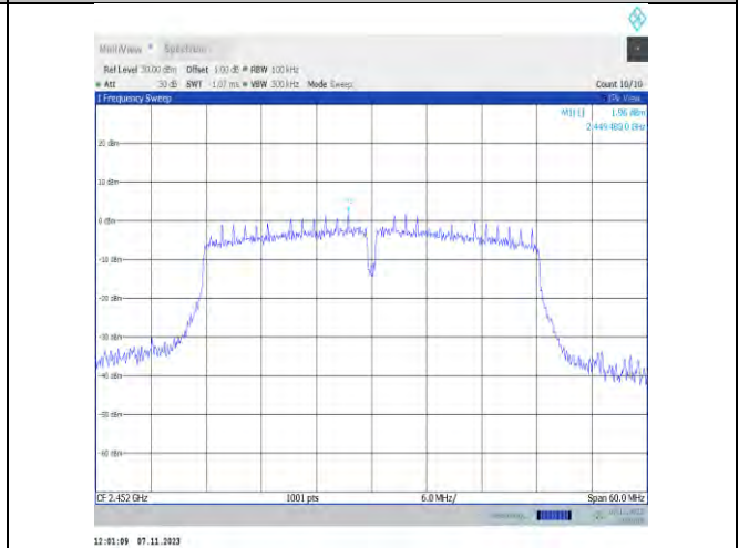
11n40SISO-Ant2-2452-0~Reference-PASS
