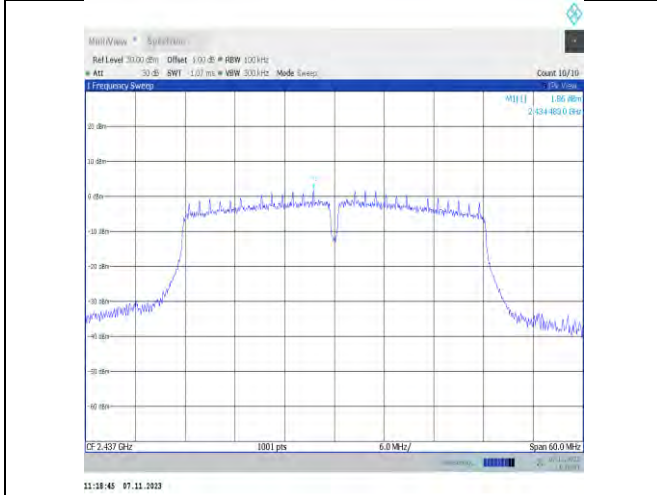
11n40SISO-Ant2-2437-0~Reference-PASS
