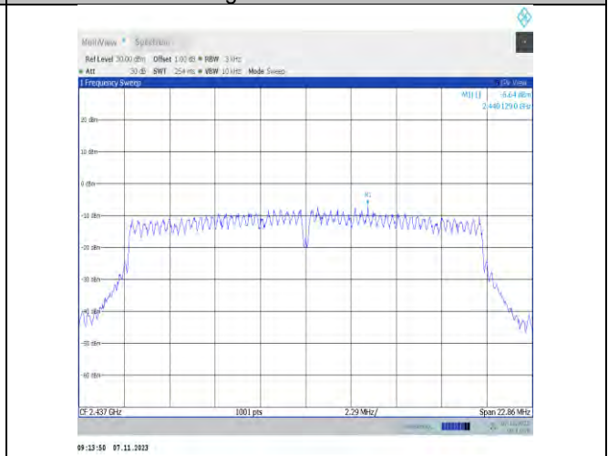
11n20SISO-Ant2-2437-PASS
