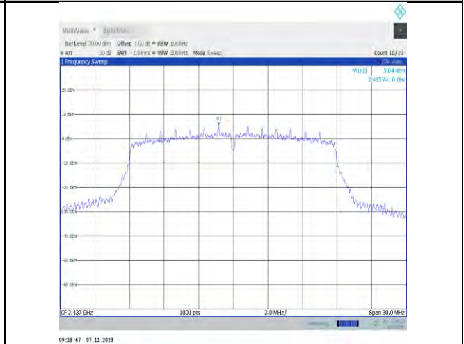
11n20SISO-Ant2-2437-0-Reference-PASS
