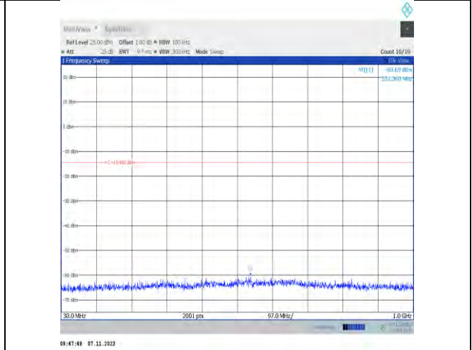
11n20SISO-Ant2-2462-30~1000-PASS
