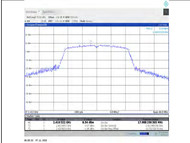
11n20SISO-Ant2-2412
