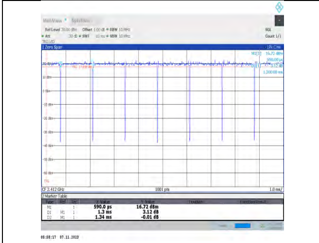
NTNV-11n20SISO-Ant2-2412
