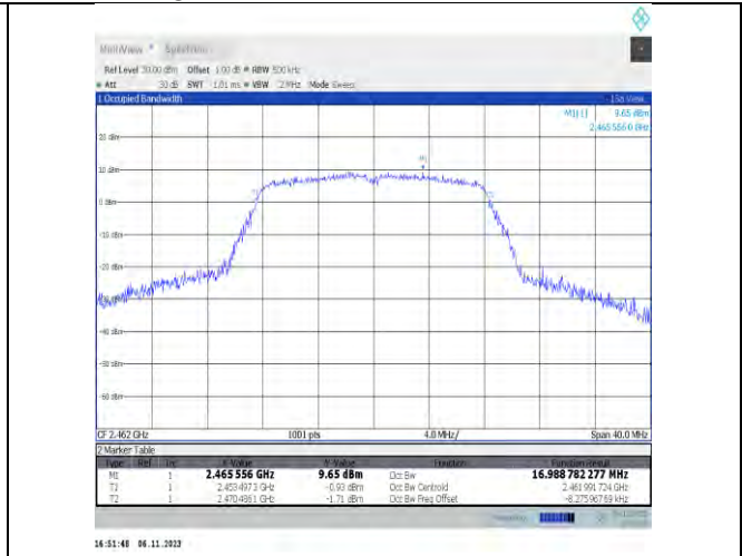
11g-Ant2-2462
