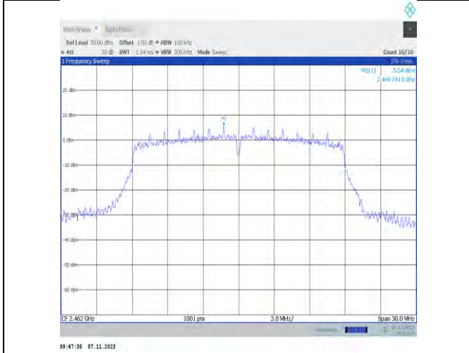
11n20SISO-Ant2-2462-0~Reference-PASS
