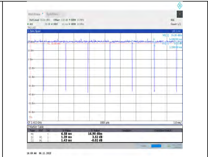
NTNV-11g-Ant2-2412
