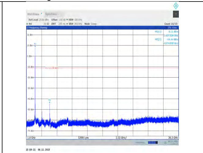
11b-Ant2-2437-1000~26500-PASS
