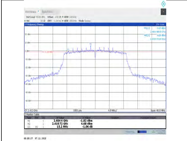
11n20SISO-Ant2-2412-PASS
