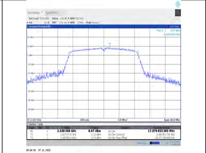
11n20SISO-Ant2-2437
