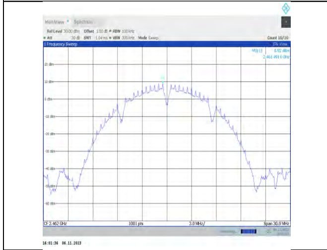
11b-Ant2-2462-0~Reference-PASS
