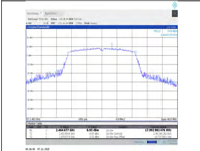
11n20SISO-Ant2-2462
