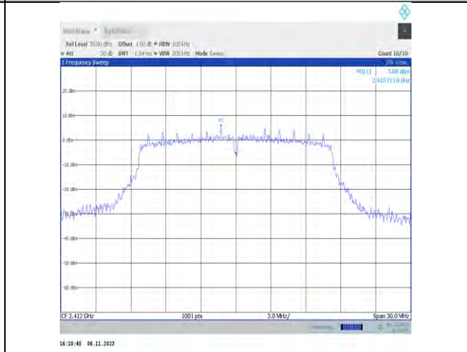
11g-Ant2-2412-0~Reference-PASS
