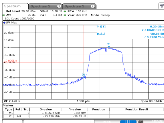
n20_2412MHz_Chain 0
