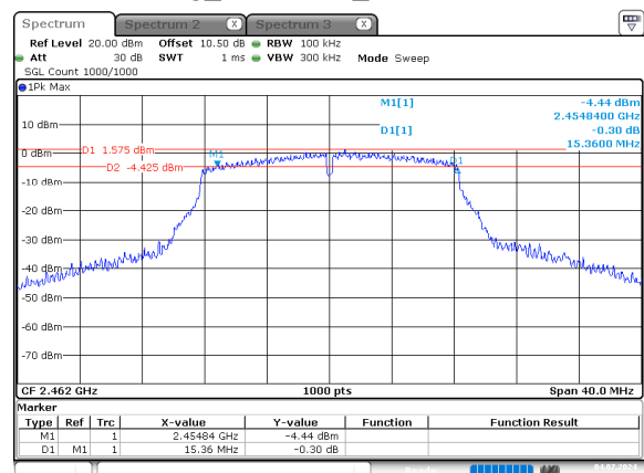
g_2462MHz_Chain 0
