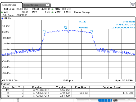
n20_5785MHz_Chain 0
