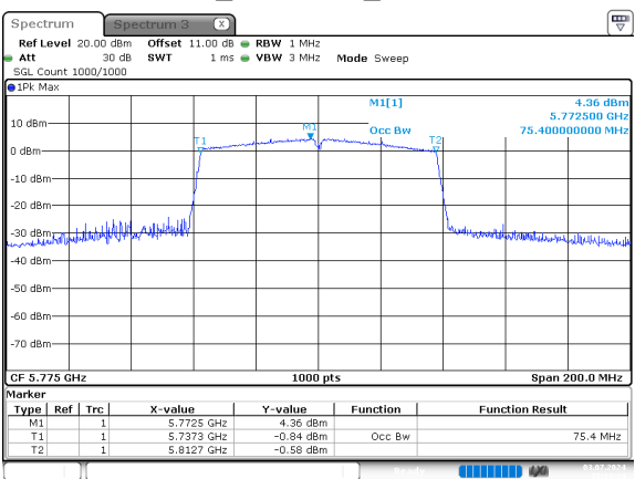
ac80_5775MHz_Chain 0
