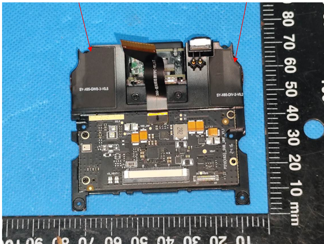
DIV Antenna(only for receive)
