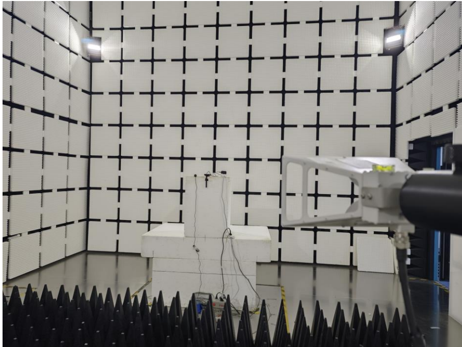
Above 1GHz-RF
