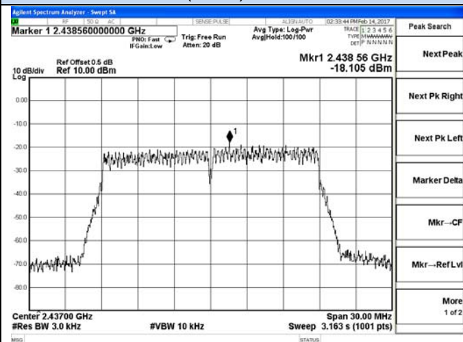
802.11n(HT20)-Middle channel
