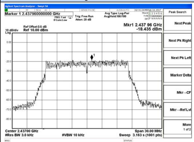
802.11g-Middle channel
