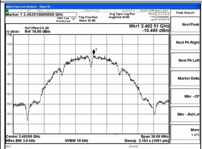
802.11b-High channel
