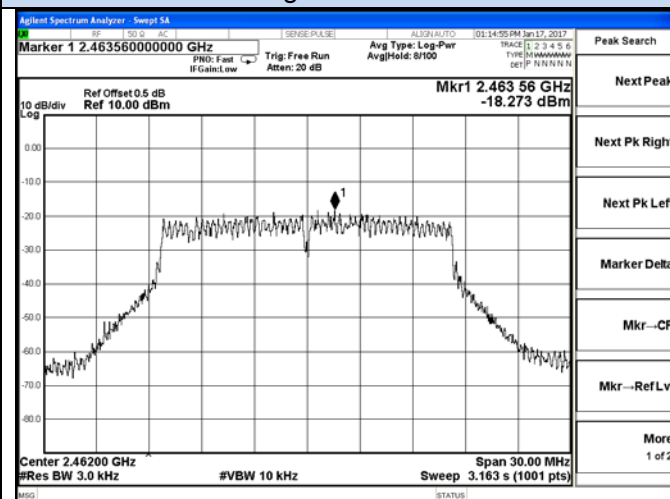
802.11g-High channel
