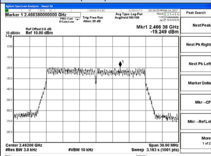
802.11n(HT20)-High channel
