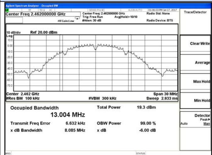
802.11b-High channel
