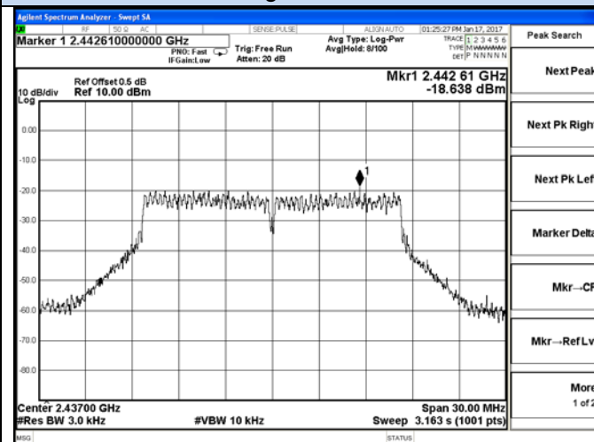
802.11g-Middle channel
