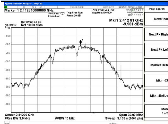
802.11b-Low channel
