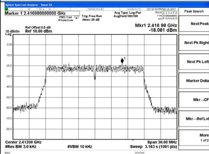
802.11n(HT20)-Low channel
