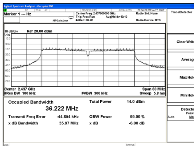
802.11n(HT40)-Mid channel
