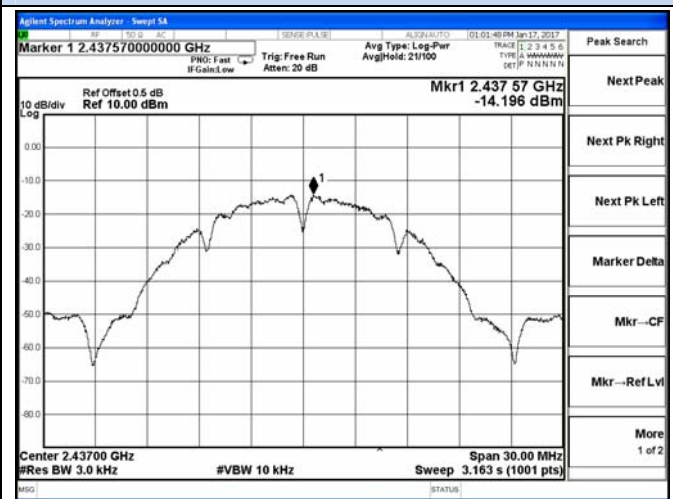
802.11b-Middle channel
