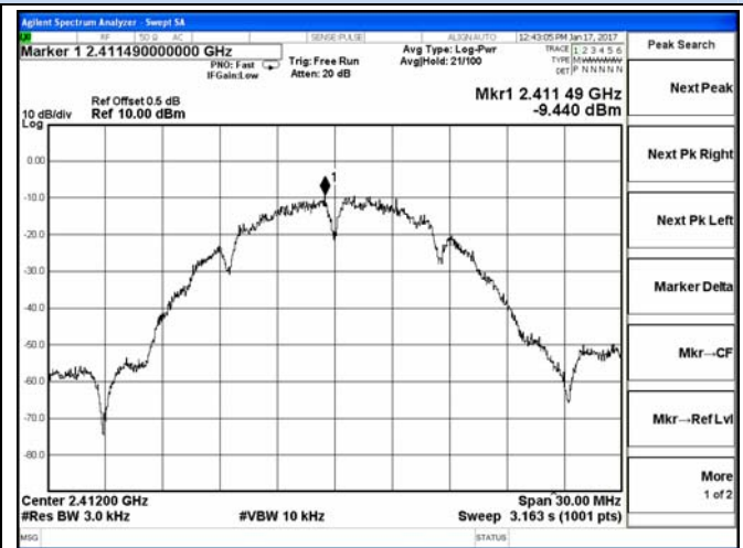
802.11b-Low channel
