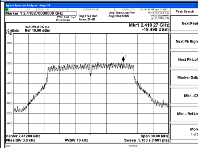
802.11g-Low channel
