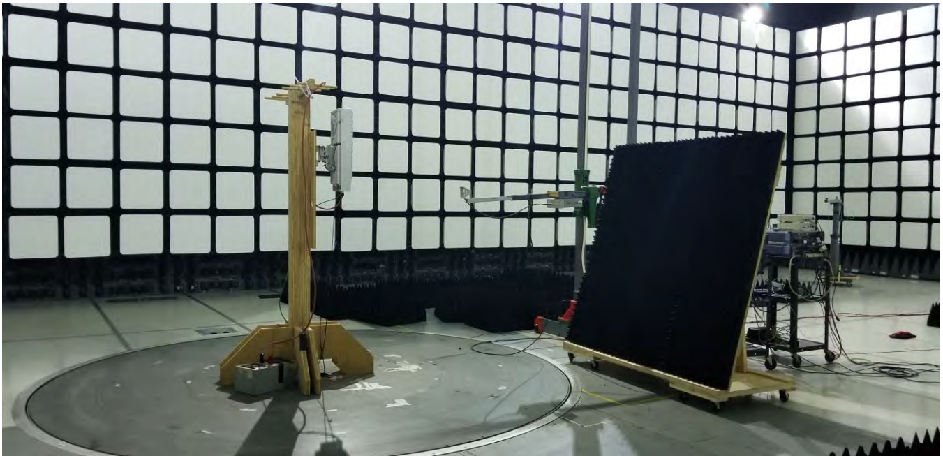
18 GHz – 26.5 GHz at 1m
