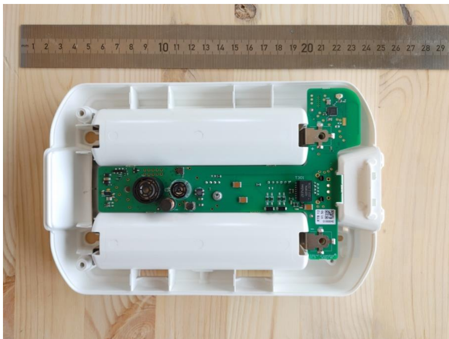
Figure 3: Photo of the PBA of INF-C365 and INF-C375, mounted inside the housing.
