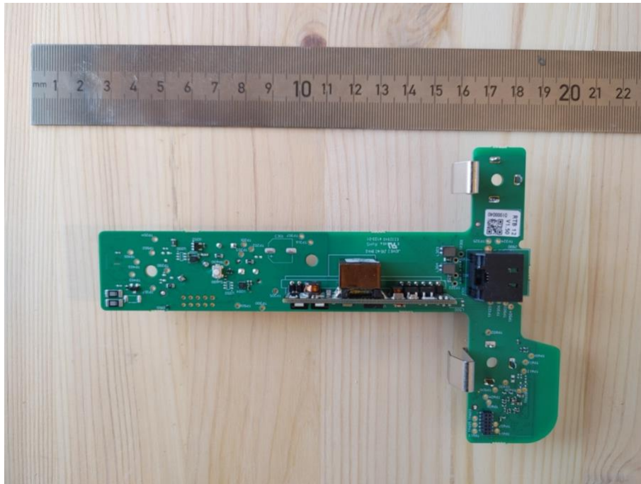
Figure 2: Photo of the PBA of INF-C365 and INF-C375, back.
