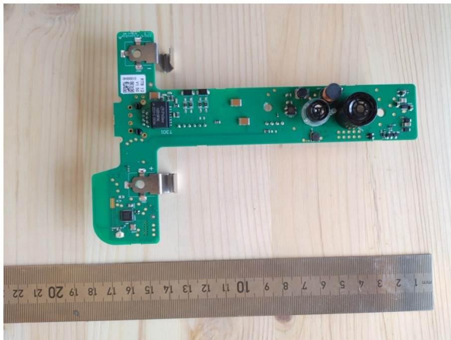
Figure 1: Photo of the PBA of INF-C365 and INF-C375, front.
