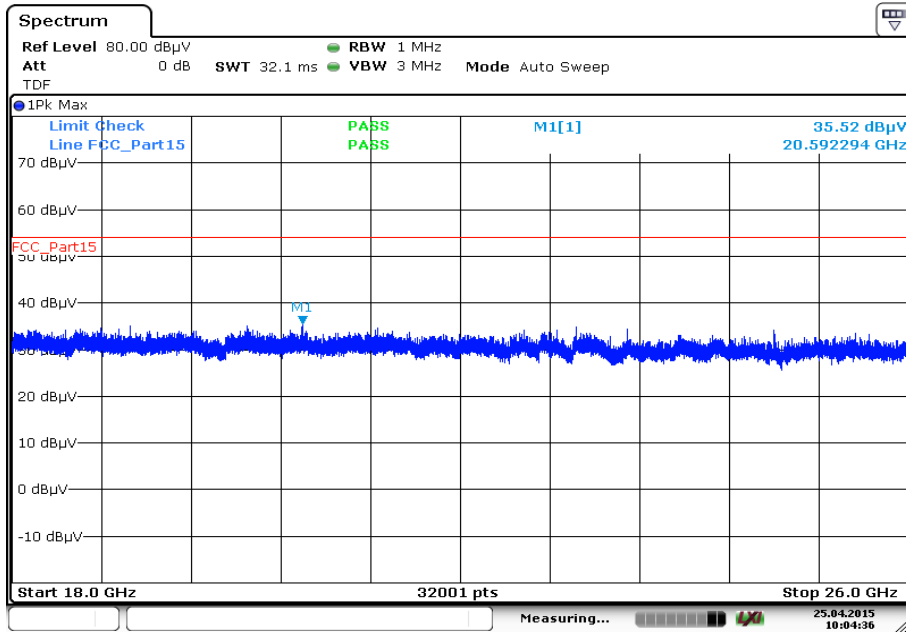
Plot 12: 18 GHz to 26 GHz, highest channel, vertical & horizontal polarization
