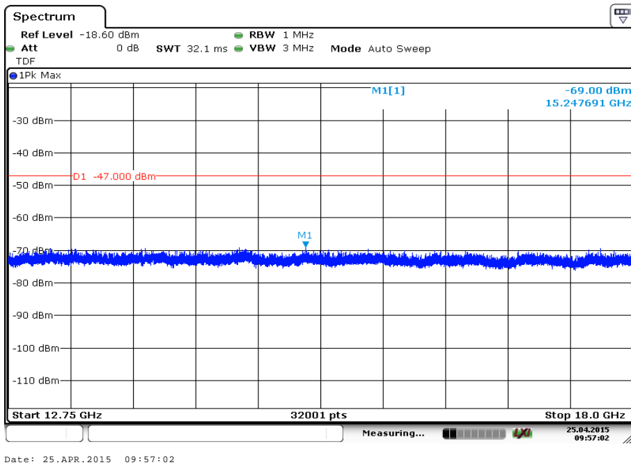
Plot 3: 12 GHz to 18 GHz, lowest channel, vertical & horizontal polarization – valid for all channels
