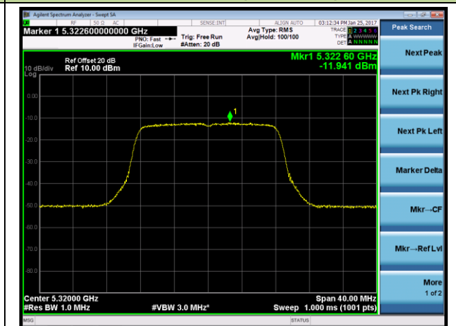
Channel 64 (5320MHz)
