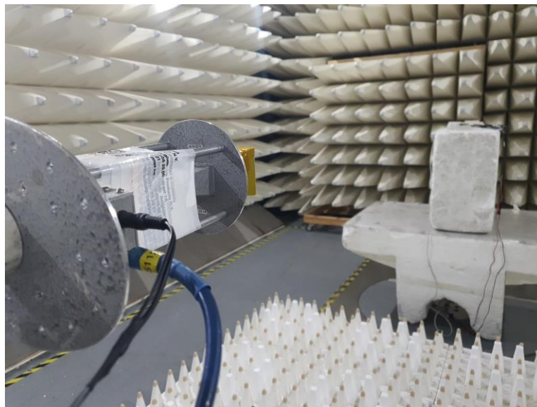
Photograph No.4 Spurious emissions measurement setup in the anechoic chamber in 18 - 40 GHz
