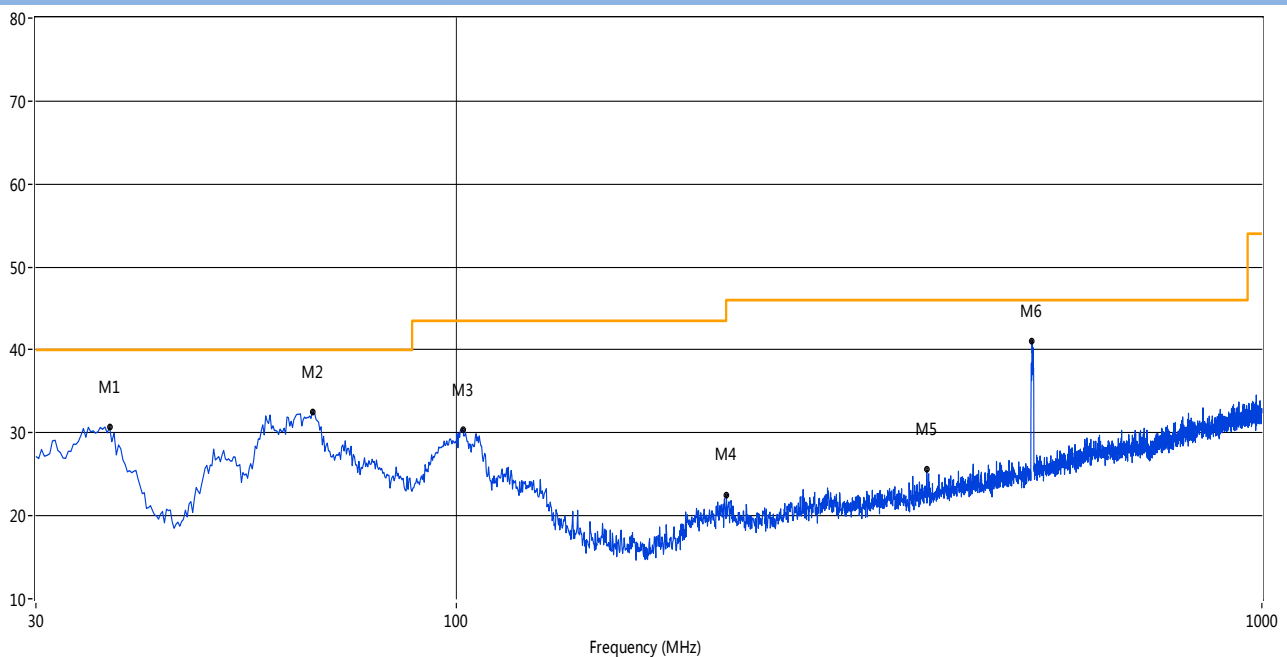
802.11b LOW CHANNEL 30MHz to 1GHz, ANT V
