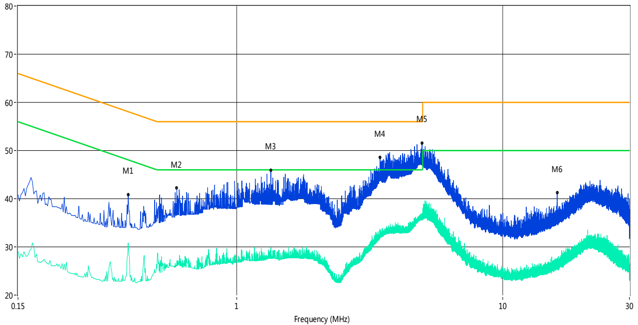
802.11g LOW CHANNEL PHASE L
