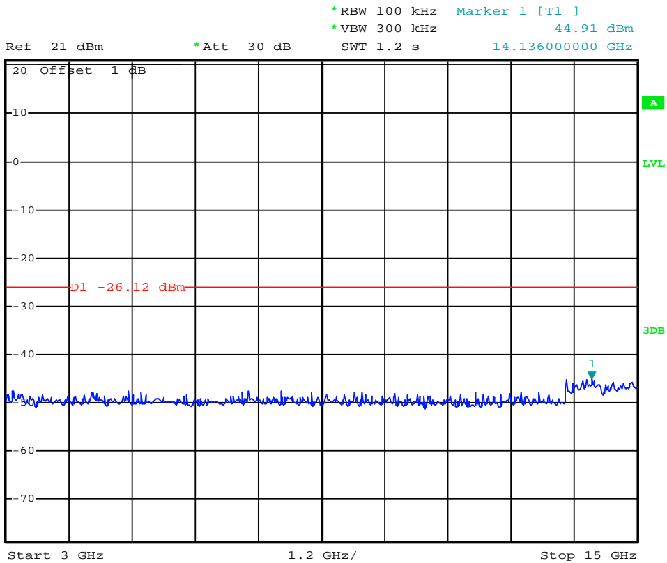
(Plot 4.6.4 A1: Channel 3: 2422MHz @ 802.11n(40MHz))
