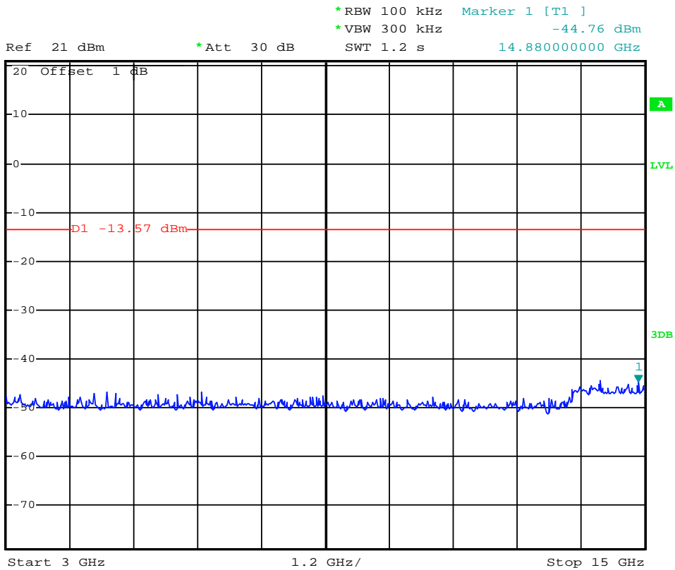
(Plot 4.6.1 B1: Channel 6: 2437MHz @ 802.11b)
