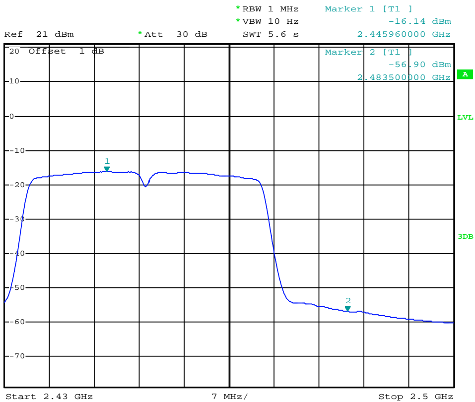
(Plot 4.5.4 A3: Channel 9: 2452MHz @ 802.11n(40MHz))
