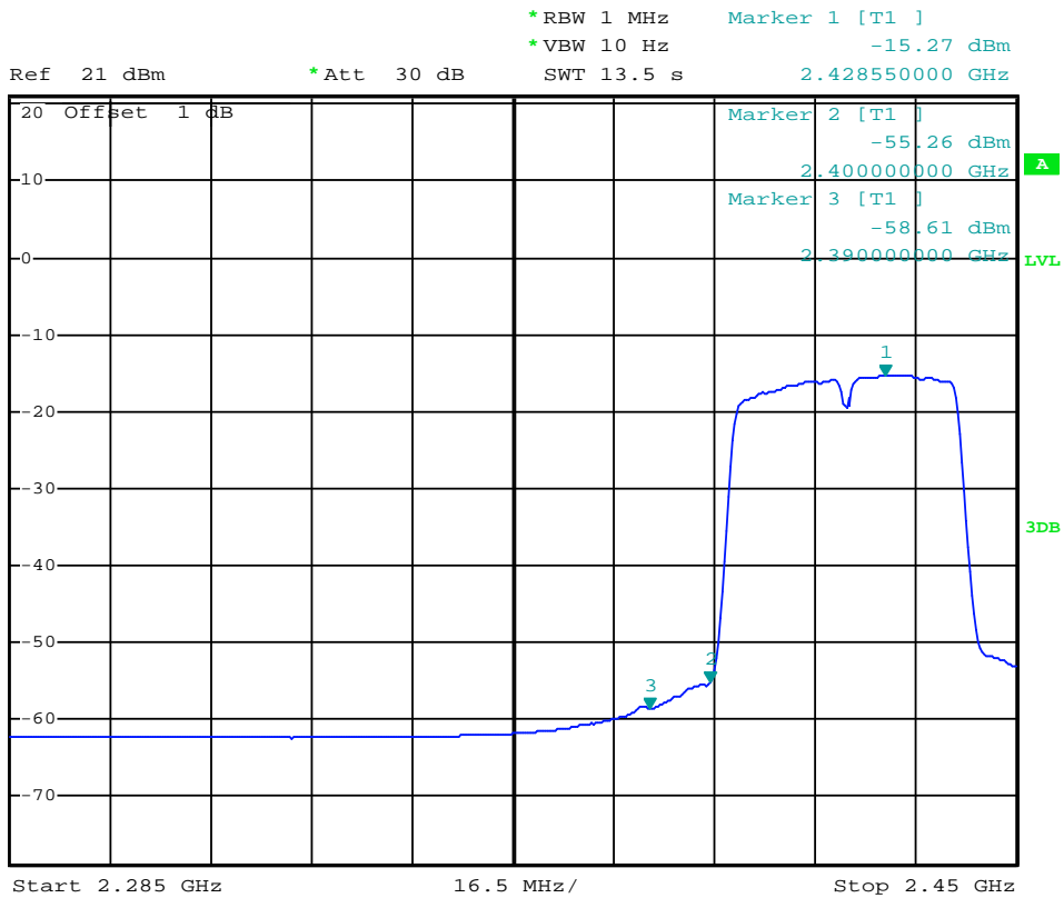
(Plot 4.5.4 A1: Channel 3: 2422MHz @ 802.11n(40MHz))
