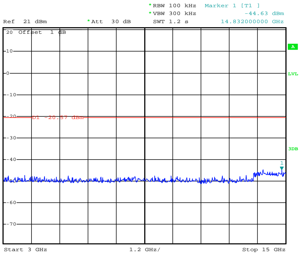
(Plot 4.6.3 A1: Channel 1: 2412MHz @ 802.11n(20MHz))
