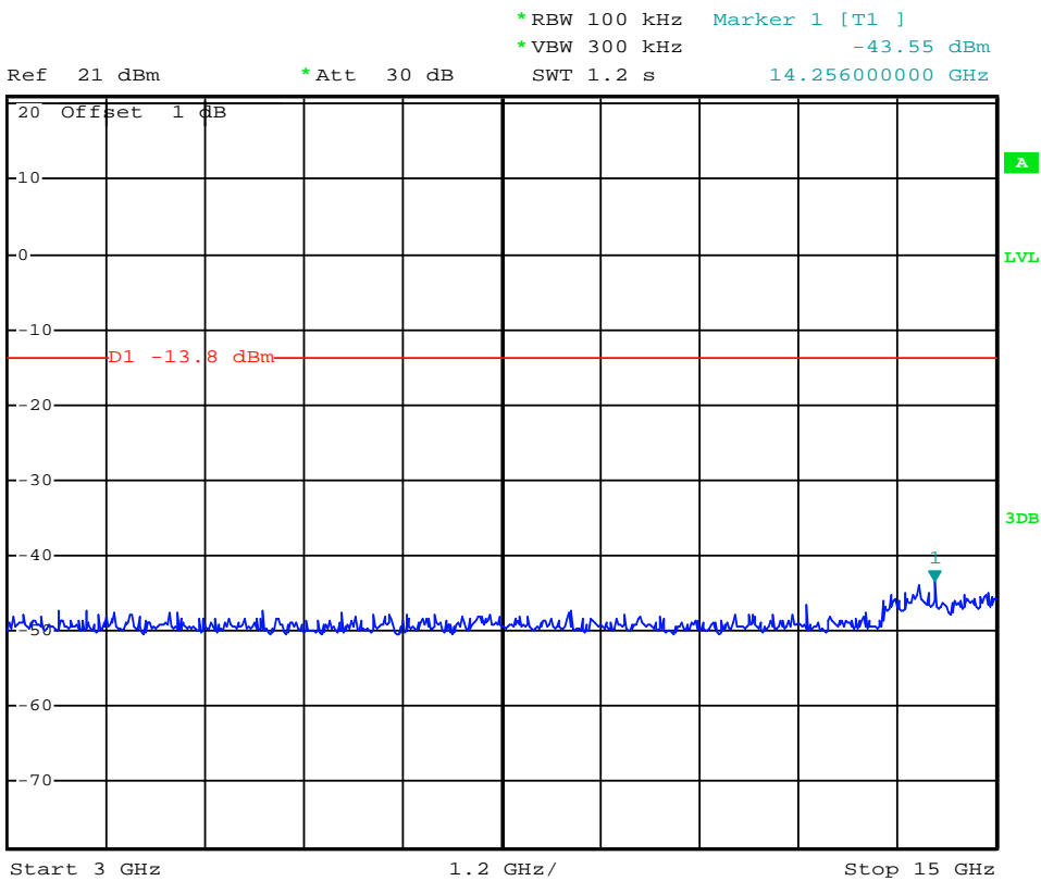
(Plot 4.6.1 A1: Channel 1: 2412MHz @ 802.11b)
