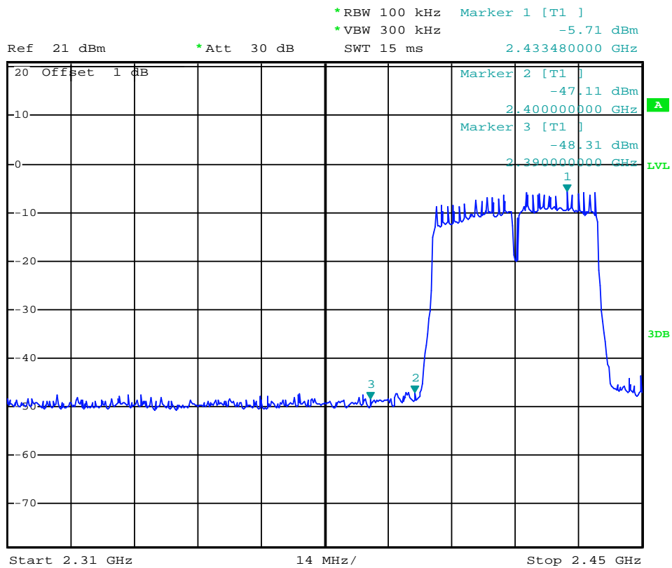
(Plot 4.6.4 A3: Channel 3: 2422MHz @ 802.11n(40MHz))
