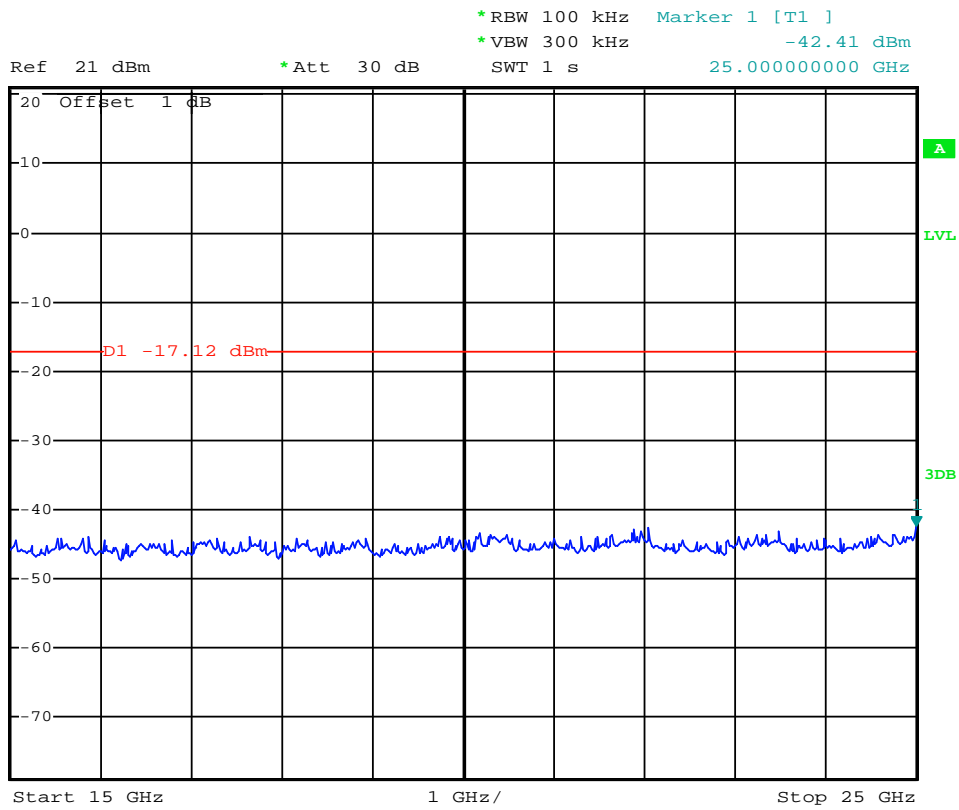
(Plot 4.6.2 C2: Channel 11: 2462MHz @ 802.11g)
