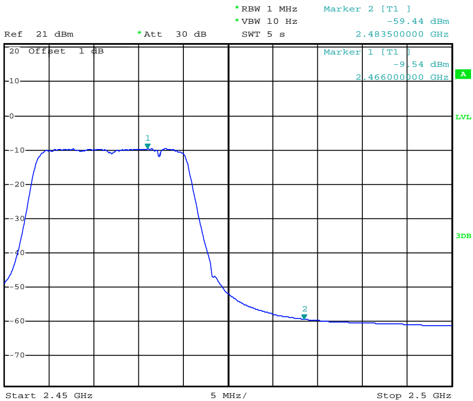
(Plot 4.5.2 A3: Channel 11: 2462MHz @ 802.11g)
