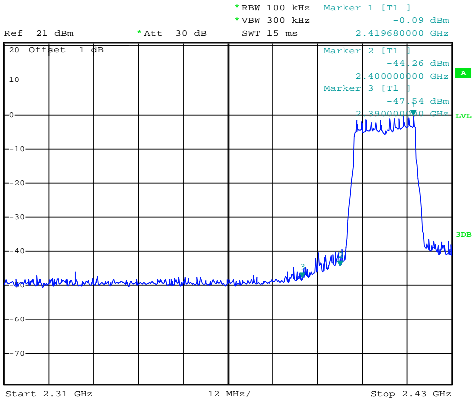
(Plot 4.6.2 A3: Channel 1: 2412MHz @ 802.11g)
