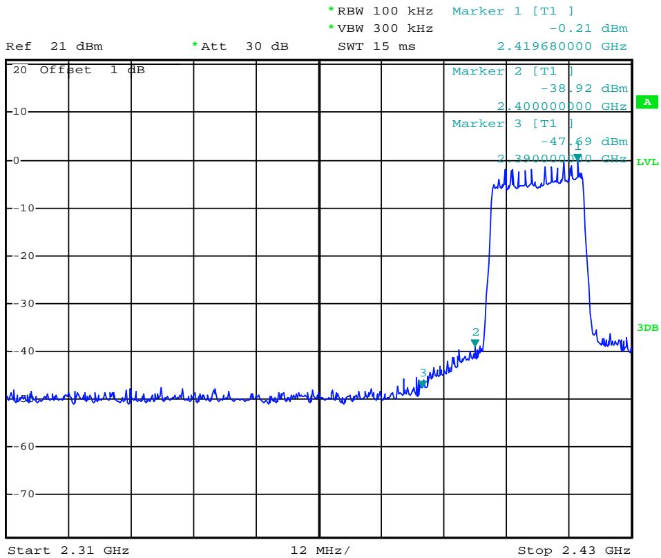
(Plot 4.6.3 A3: Channel 1: 2412MHz @ 802.11N(20MHz))
