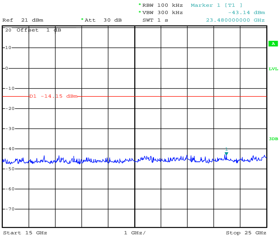
(Plot 4.6.1 C2: Channel 11: 2462MHz @ 802.11b)
