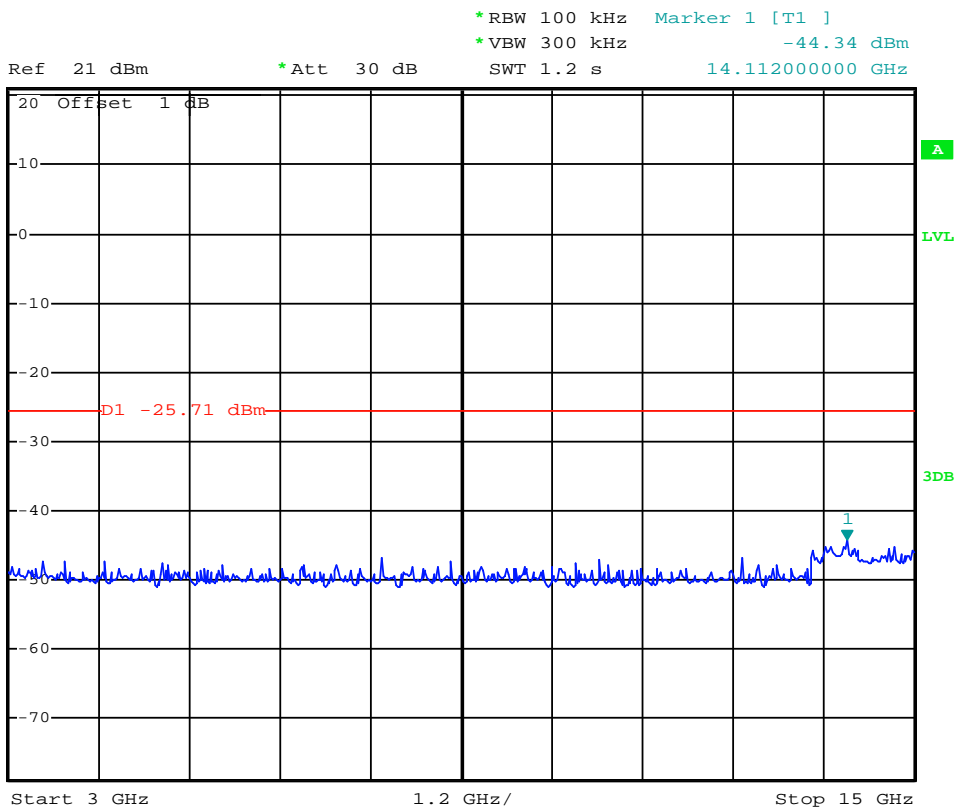
(Plot 4.6.4 B1: Channel 6: 2437MHz @ 802.11n(40MHz))
