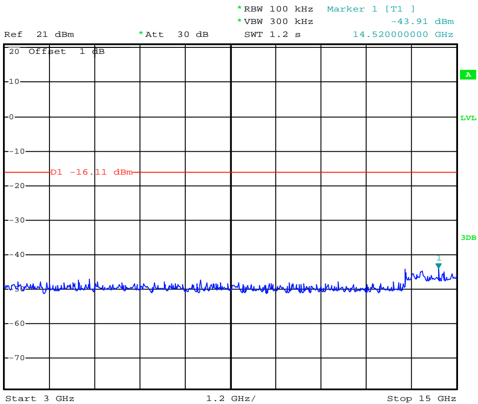
(Plot 4.6.2 B1: Channel 6: 2437MHz @ 802.11g)
