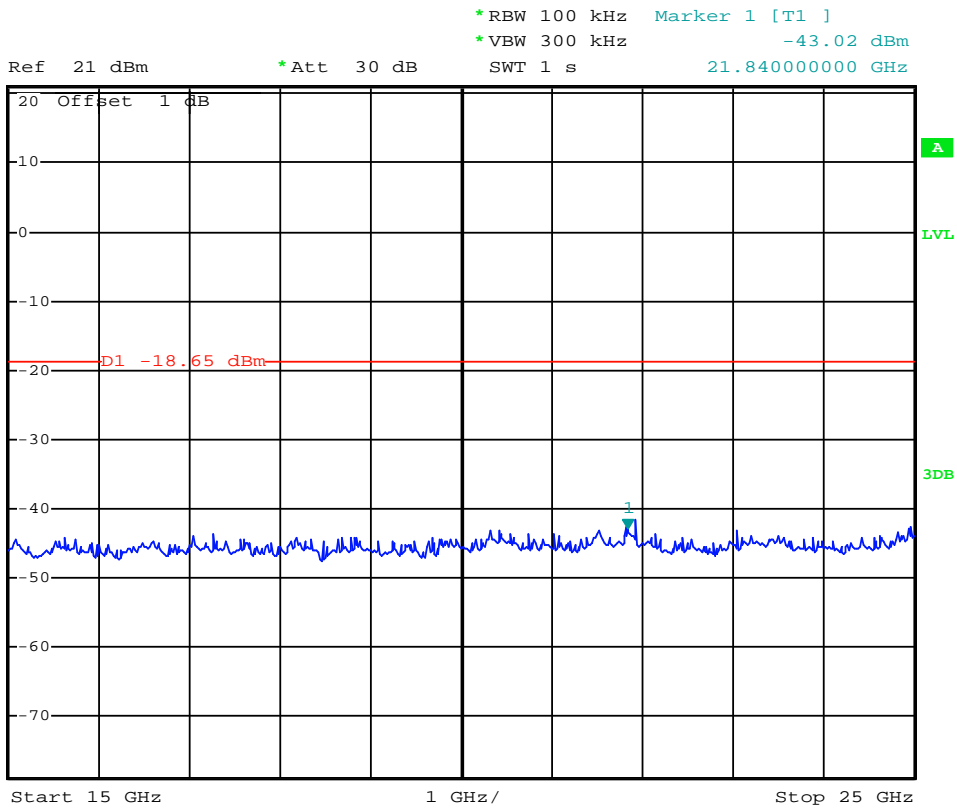
(Plot 4.6.3 C2: Channel 11: 2462MHz @ 802.11N(20MHz))
