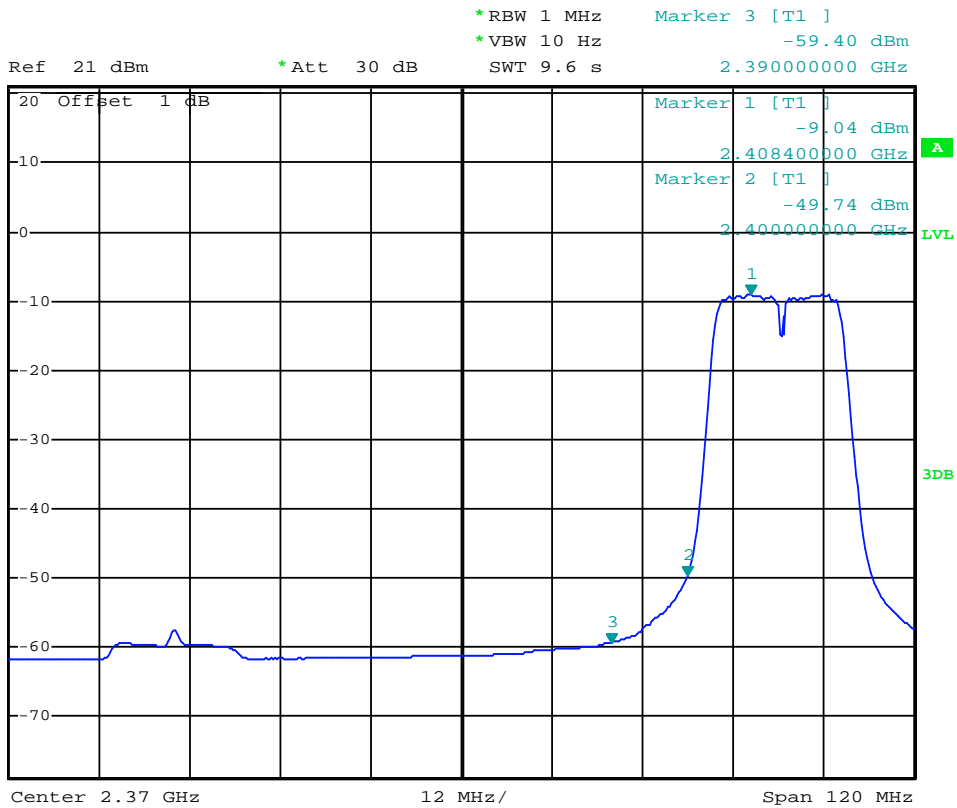
(Plot 4.5.2 A1: Channel 1: 2412MHz @ 802.11g)
