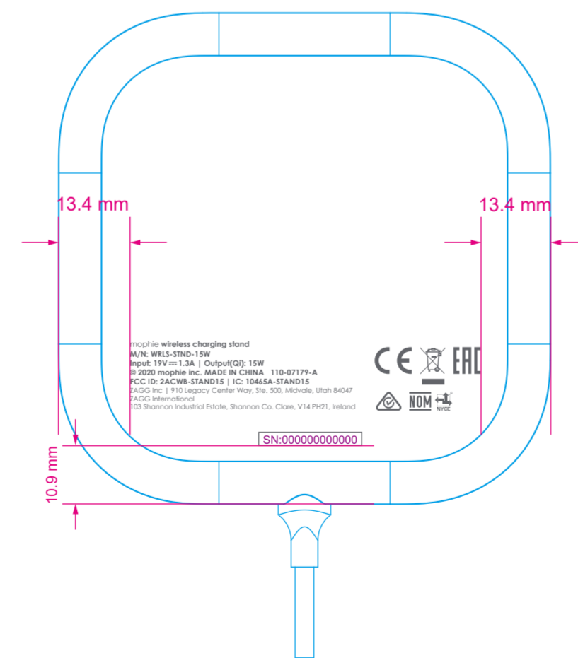
bottom view
