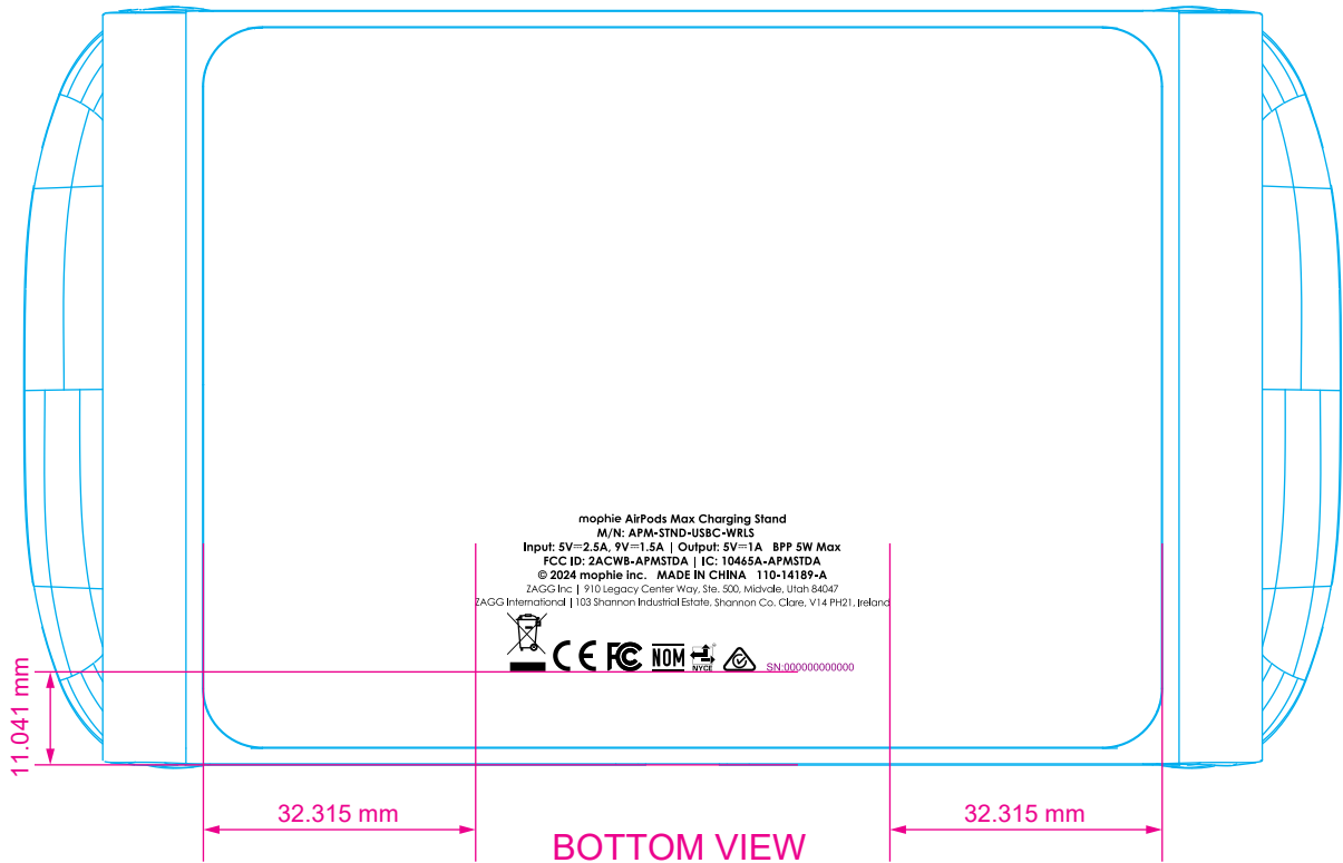
BOTTOM VIEW
