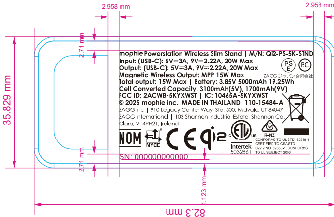
KICK STAND BACK VIEW
