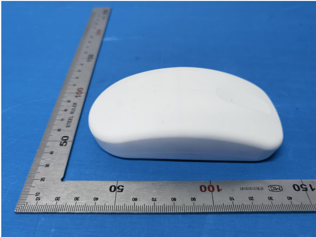
VIEW-1 OF EUT( 3-Button Scroll)
