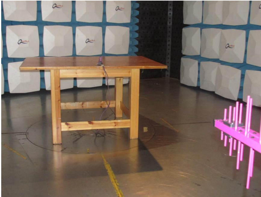
Photograph 3: Radiated Measurements
