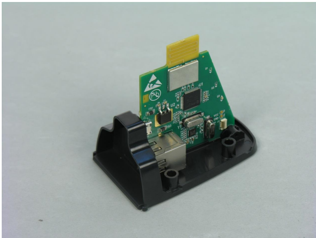
Figure 1 - Gateway Internal
