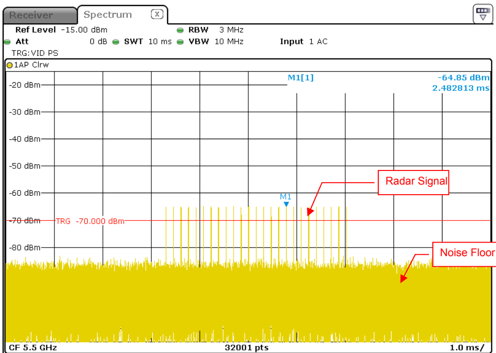
Radar Signal 2
