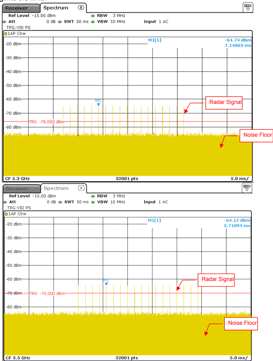
Radar Signal 0
