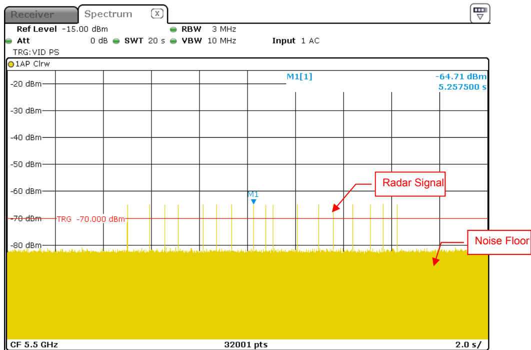
Radar Signal 5
