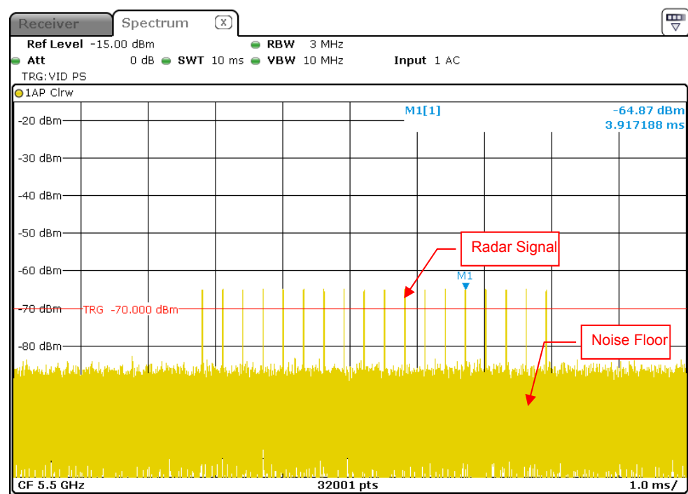
Radar Signal 3
