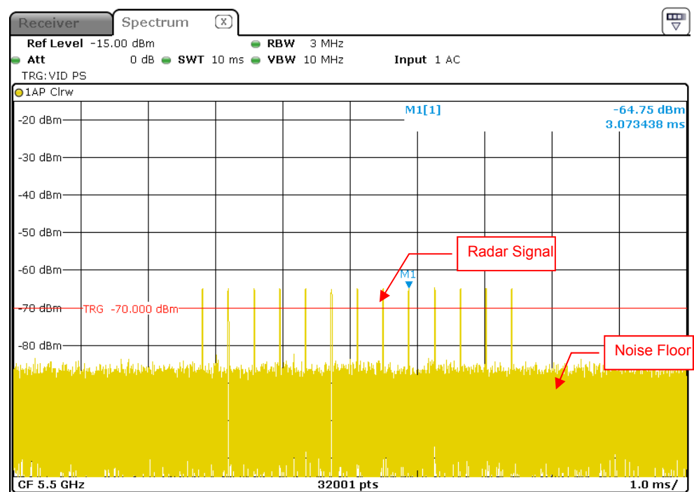
Radar Signal 4
