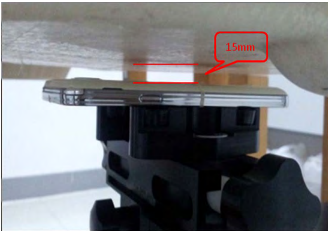
Body Worn
