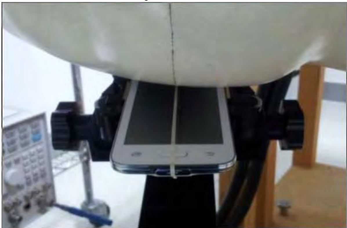
Right Tilt(15° )
