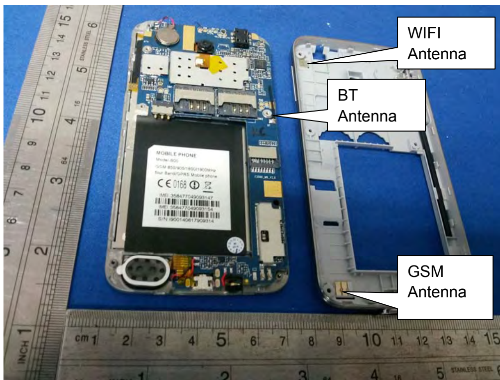
Antenna Location
