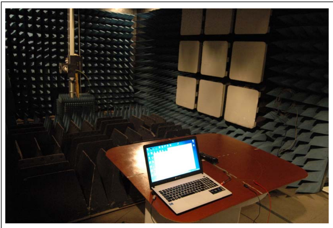
Radiated emission Test
