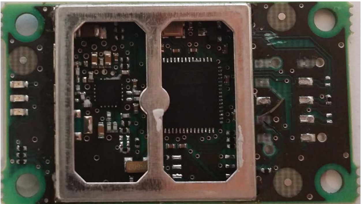
Figure 3: EUT – Top without shielding (View 2)
