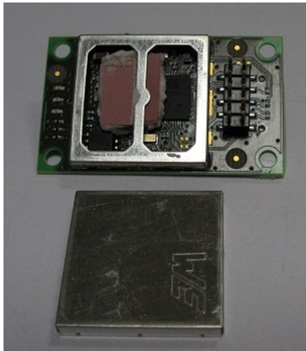
Figure 2: EUT – Top without shielding (View 1)
