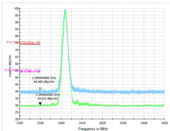
Test Mode: \pi/4 DQPSK-Low
