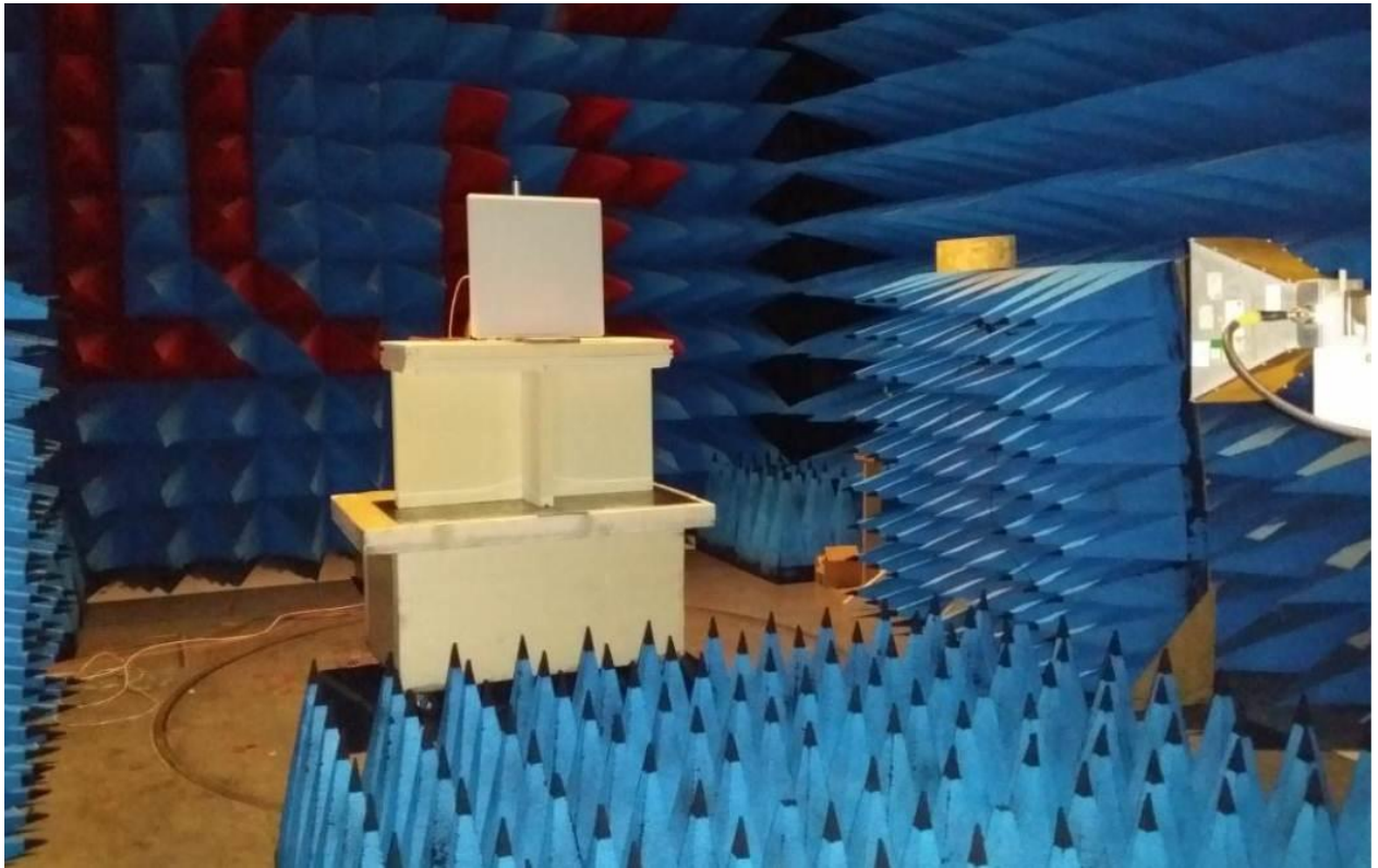
Test setup for radiated field strength (above 1GHz)
