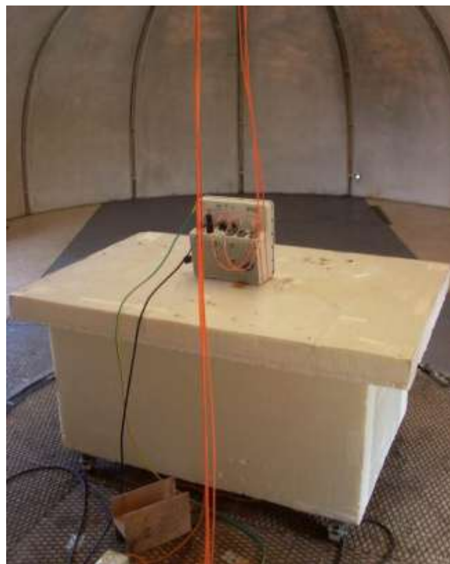
Test setup for radiated field strength
