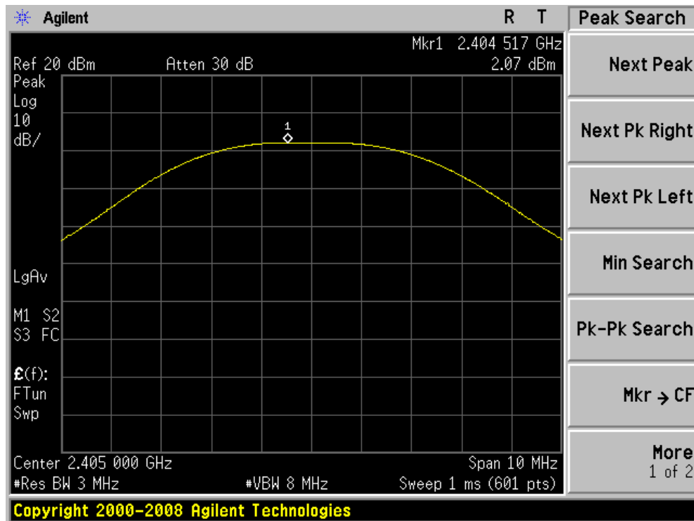
Peak output Power plot on channel 7
