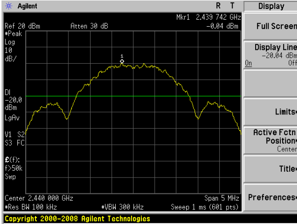
GFSK on channel 7
