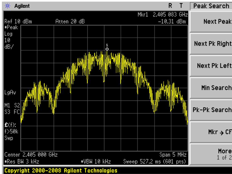
Power spectral density plot on channel 7
