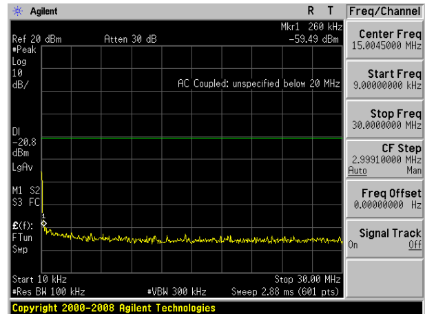
GFSK on channel 1
