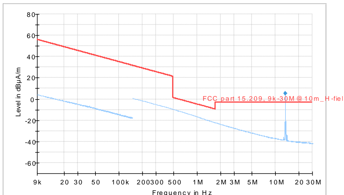
Diagram, Peak overview sweep, 0.009 – 30 MHz at 10 m distance.
