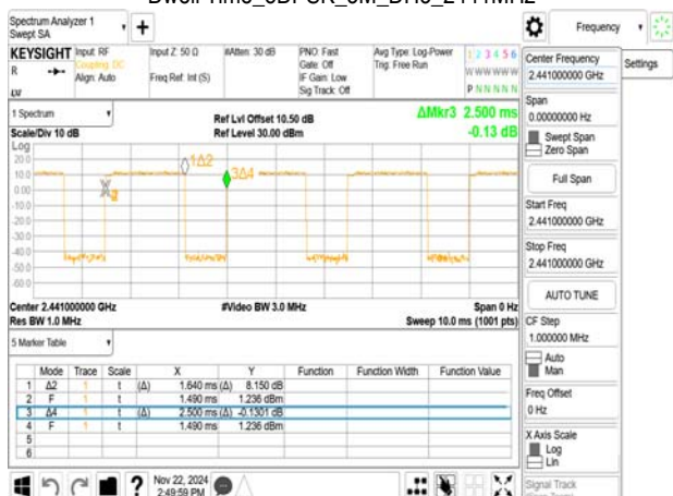
Dwell Time_8DPSK_3M_DH5_2441MHz
