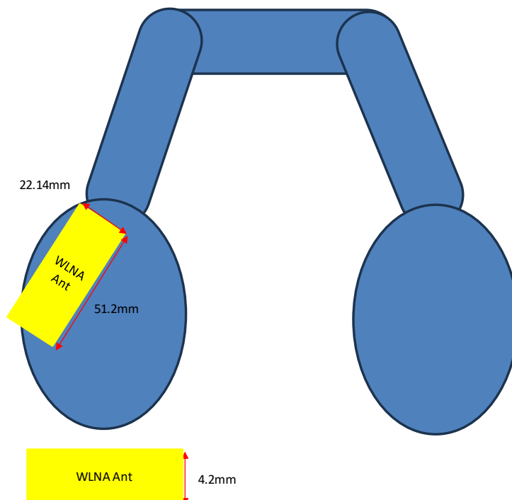
Photograph 23. Antenna position of EUT
