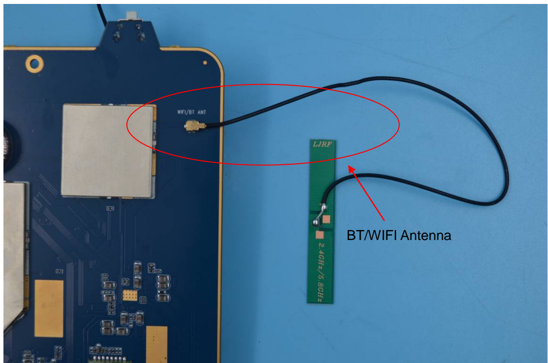
4. Antenna view
