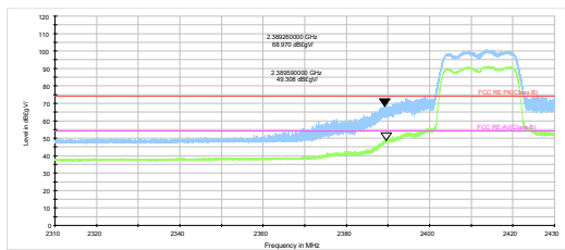
802.11n HT20-Channel 1 Peak+ Average
