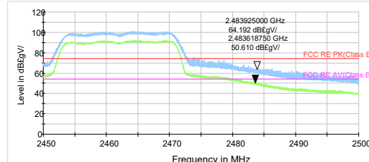
802.11n HT20-Channel 11 Peak+ Average
